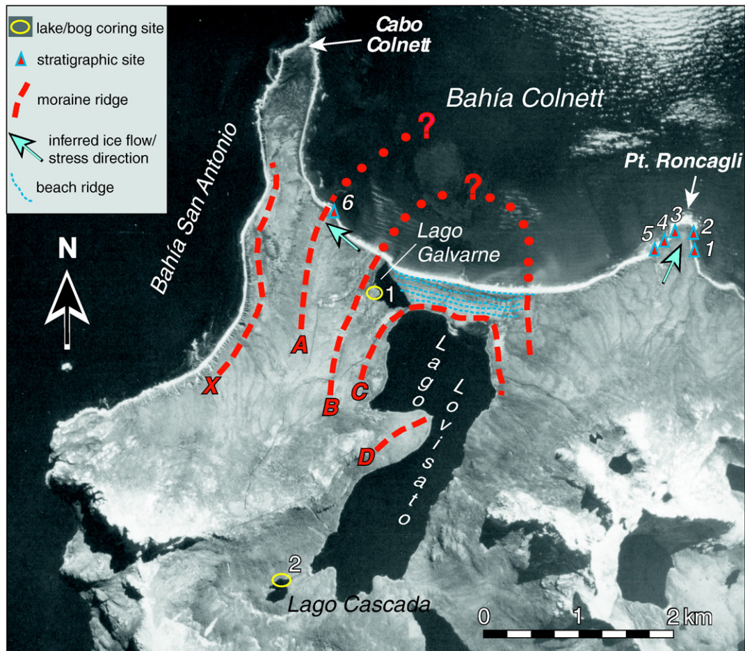
Figure 4. Aerial photo image of the Bahía Colnett area. The position of ice-marginal moraines, investigated glacialigenic stratigraphic sites and bog/lake coring sites are indicated.
