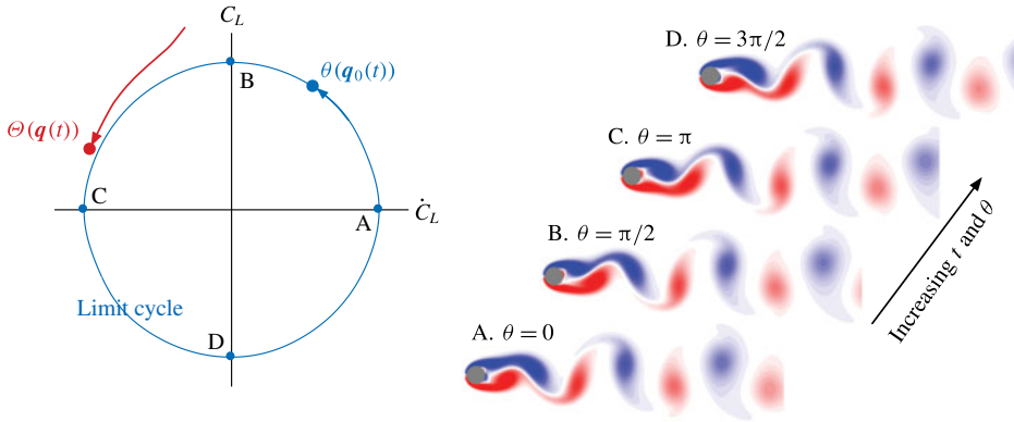
FIGURE 1. Definition of phase \theta and phase function \Theta with C_L and \dot{C}_L for cylinder flow at a Reynolds number of Re = 100 . Vorticity fields are shown at representative phases.
