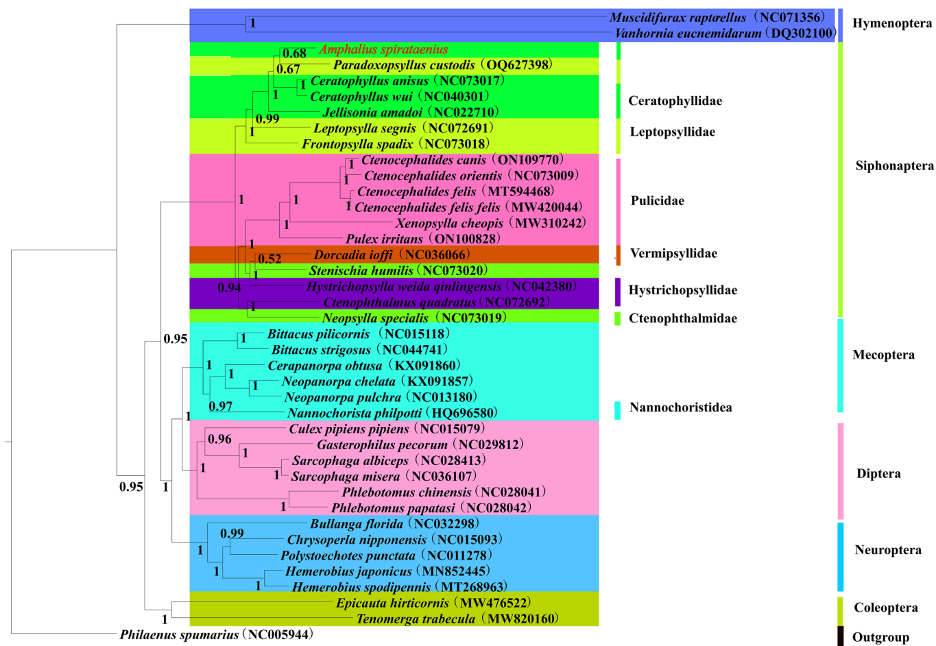
Figure 5. Phylogenetic tree of 40 insect species was constructed using Bayesian methods with Philaenus spumarius as the outgroup and node values as posterior probability values (PP). Amphilus spirataenius was labelled in red.
