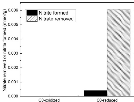
Figure 1. Nitrate removal and nitrite formation by unaltered (oxidized) (std. dev. = ± 0) and reduced Na + -SWa-1 (sample C0). (std. dev. = ± 0.006 mmol nitrate/g and 0.0004 mmol nitrite/g).
