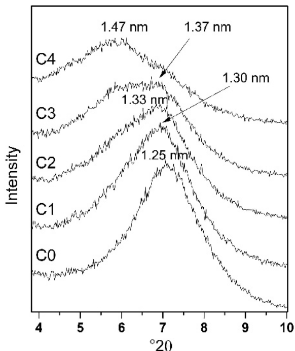
Figure 3. XRD patterns of oxidized or unaltered (oxidized) samples C0 to C4.
