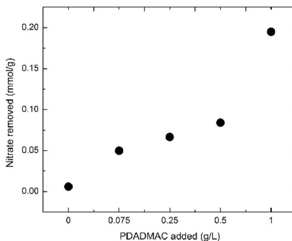
Figure 6. Nitrate removed from solution by reduced poly-DADMAC-SWa-1 (std. dev. (mmol/g): C0 = 0.006, C1 = 0.001, C2 = 0.005, C3 = 0.003, C4 = 0.006).
