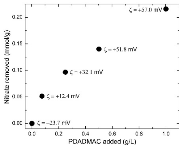
Figure 5. Zeta ( \zeta ) potential (std. dev. = \pm 7 mV) measurements and amount of nitrate removed from solution by the oxidized forms of the poly-DADMAC-SWa-1 samples C0 to C4. (std. dev. (mmol/g): C0 = 0, C1 = 0.0036, C2 = 0.0079, C3 = 0.0035, C4 = 0.0024).
