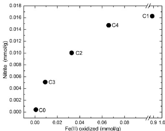
Figure 7. Nitrite formation (mmole nitrite in solution per g of poly-DADMAC-SWa-1) as a function of Fe(II) oxidation (mmole Fe(II) per g of poly-DADMAC-SWa-1) in reduced poly-DADMAC-SWa-1 (nitrite std. dev. (mmol/g): C0 = 0.0004, C1 = 0.0140, C2 = 0.0025, C3 = 0.0010, C4 = 0.0070; Fe(II) std. dev. (mmol/g): C0 = 0.090, C1 = 0.200, C2 = 0.001, C3 = 0.009, C4 = 0.027).
