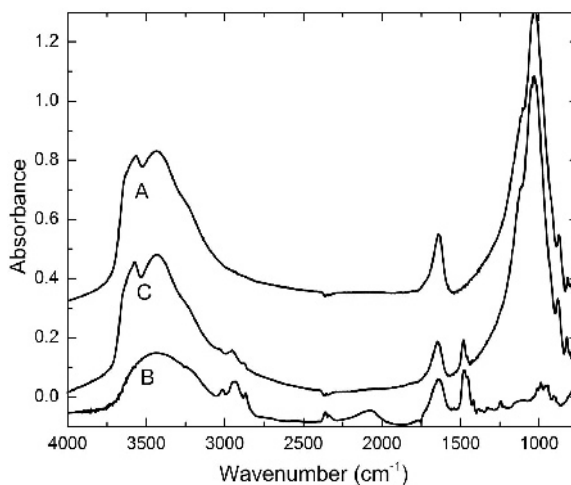
Figure 4. FTIR spectra of (A) \text{Na}^+ -SWa-1, (B) pure poly-DADMAC, and (C) poly-DADMAC-SWa-1 sample C4, all in the unaltered (oxidized) state.
