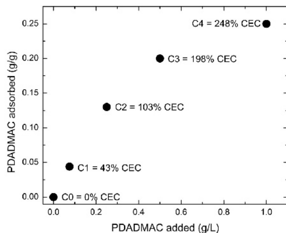
Figure 2. Adsorption of poly-DADMAC (0–1 g/L added) on unaltered (oxidized) SWa-1 (1.67 g/L) smectite samples C0 to C4, expressed as both the gravimetric amount adsorbed (std. dev. = \pm 0.03 g/g) and the fraction of CEC adsorbed.
