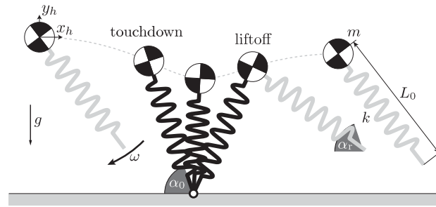
Fig. 2. The SLIP model with swing-leg retraction. The model consists of a point mass body and a massless spring leg. At liftoff, the leg instantaneously assumes angle \alpha_r with respect to the ground and begins rotating at rate \omega . The leg angle at touchdown \alpha_0 depends on the time between liftoff and touchdown.
