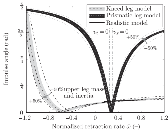
Fig. 9. The effect of the normalized swing-leg retraction rate \bar{\omega} on the impulse angle for prismatic leg, knead leg, and realistic models. Impulse angle, or the magnitude of the angle between the impulse and vertical, is defined as |\text{atan}(I_x/I_y)| , where I_x and I_y are the horizontal and vertical components of the impulse vector respectively. A lower value corresponds with an impulse closer to vertical and less slipping at touchdown. The meaning of strokes and shading are the same as in Figs. 6 and 8
