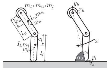
Fig. 5. Kneed leg model, a simplification of the realistic model in which the mass of the opposing leg and the torso are lumped into a point mass at the hip.
