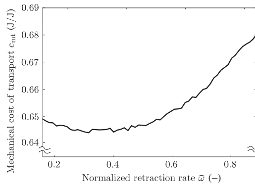
Fig. 7. The effect of the normalized retraction rate \bar{\omega} on the mechanical cost of transport of limit cycle running under the hand-tuned controller.
