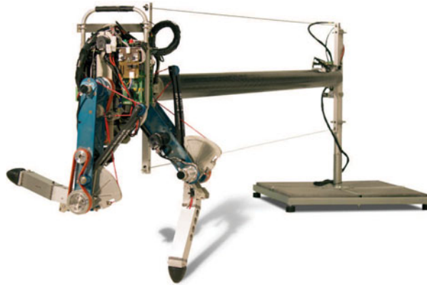
Fig. 1. Running robot “Phides”. This robot consists of a torso and two kneed legs with small, spherical feet. The robot is attached to a boom with a parallelogram mechanism to achieve planar behavior. The two hip joints are directly actuated by DC motors in the torso. The two knee joints are actuated by DC motors with a spring in series (torsion bar inside the knee shaft) as well as a spring in parallel (leaf spring with pulley mechanism).
