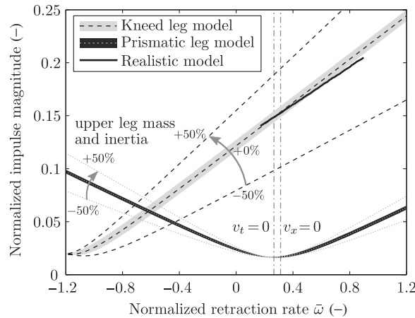
Fig. 8. The effect of the normalized swing-leg retraction rate \bar{\omega} on the normalized touchdown impulse magnitude for prismatic leg, knead leg, and realistic models. The meaning of strokes and shading are the same as in Fig. 6.
