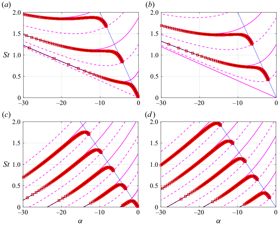
Figure 15. Prediction of cut-on frequency–wavenumber pairs of totally reflected acoustic waves based on the wavelength of standing waves. Solution for symmetric (a,c) and anti-symmetric (b,d) modes for M = 0.8 (a,b) and 1.2 (c,d), with T = 1 . Dotted (.) blue lines indicate the sonic line, magenta solid (-) and dashed (- -) lines indicate the soft- and hard-wall duct dispersion relations, black dash-dot (-.-) lines indicate the guided-jet mode obtained from the DVS dispersion relation and red squares ( \square ) show the frequencies obtained from the standing-wave argument using the SVS.
