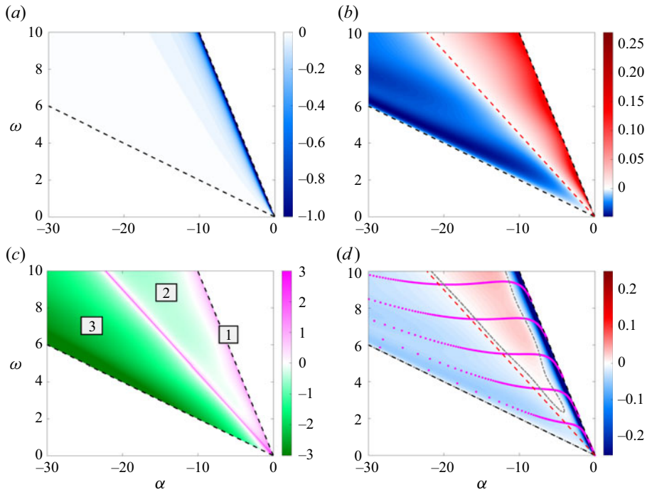
Figure 17. Streamwise energy flux for waves travelling in the quiescent region (a) and flow region (b) as a function of frequency and wavenumber for M = 0.8 . Logarithms of the absolute value of the ratio between the fluxes (c) and the total-energy flux (d) are also shown. Black dashed lines indicate wavenumber–frequency pairs where total reflection occurs, and the red dashed line indicates the phase speed associated with no energy propagation in the streamwise direction. Grey dot-dashed lines indicate regions where the flux is zero, and magenta dots represent the dispersion relation of the guided-jet mode.
