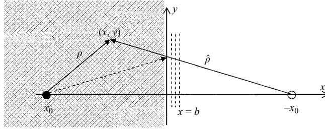
FIGURE 12. Geometrical interpretation of the asymptotic result (B 5). The point source is denoted by a solid circle and its image by an open circle. The region of depth variation is shown by using dashed lines to indicate the parallel bottom contours.
