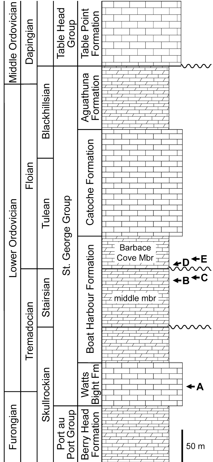
Figure 2. Generalized stratigraphic section of the St. George Group in western Newfoundland (based on Knight et al., 2008, fig. 2; with updated chronostratigraphy in Boyce et al., 2013, fig. 2). The North American Skullrockian through Blackhillsian stages comprise the Ibexian Series. Besides the contact between the St. George Group and the overlying Table Head Group, there are two significant regional disconformities within the Boat Harbour Formation (shown with wavy lines). The middle member and Barbace Cove Member of the Boat Harbour Formation are labeled, but other members are not. Lithologic symbols: rectangles = limestone; right trapezoids = interbedded limestone and dolostone. Stratigraphic positions of Amsassia and Reptamsassia n. gen. are marked with arrows (geographic locations are shown in Fig. 1.2): A, Amsassia terranovens and Amsassia? sp. A, ~26–33 m above base of Watts Bight Formation at Green Head; B, Amsassia divers a and Amsassia? sp. B, ~18 m below top of middle member in Boat
