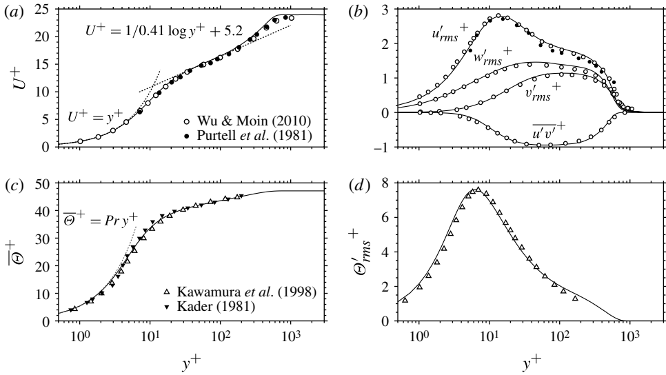
FIGURE 2. Turbulence statistics of the unheated case ( T_w = T_\infty ) at Re_\theta = 1840 . (a) The mean streamwise velocity; (b) r.m.s. of turbulence intensities and the Reynolds shear stress normalized by u_\tau . (c) Mean scalar and (d) r.m.s. of scalar fluctuation. Profiles in (c,d) are normalized by the friction temperature.
