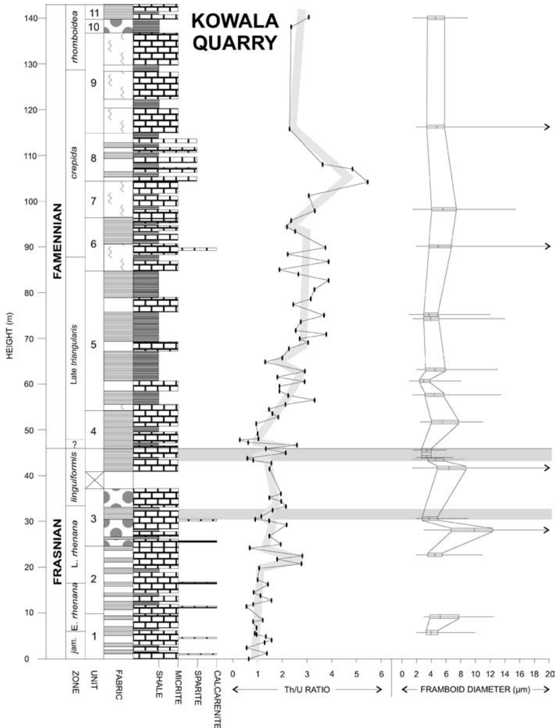
Figure 5. Graphic log of the F-F boundary beds at Kowala, showing box-and-whisker plots of frambooid diameters, and Th/U ratios derived from gamma-ray spectrometry data. Conodont zonal boundaries are from Szulcowski (1996) and Racki & Baliński (1998). For legend see Figure 3.
