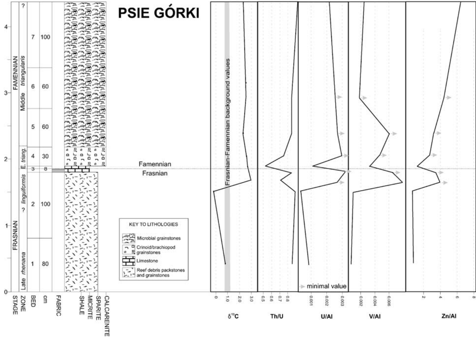
Figure 9. Graphic log of the F–F boundary beds from the forereef location of Psie Górki, Kielce, showing associated fluctuations in C isotopes and redox-sensitive trace element ratios, showing a change to oxygen-restricted deposition in the Late linguiformis Zone.
