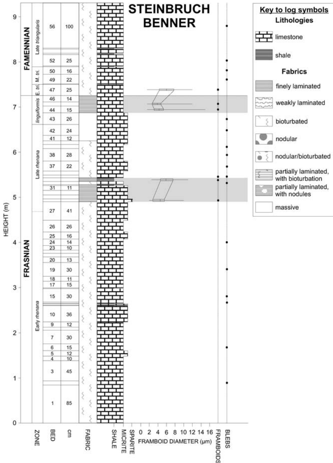
Figure 3. Graphic log of Steinbruch Benner section showing box-and-whisker plots of frambooid diameters (the ‘whiskers’ depict minimum and maximum diameters, the ‘box’ depicts the 25th and 75th percentile and the central line the median average). Conodont zonation based on Schindler (1990).
