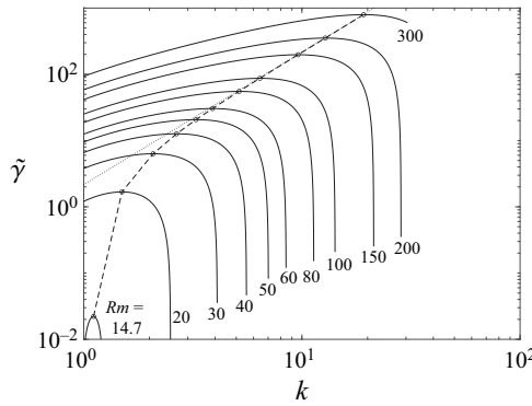
Figure 4. Plot of \tilde{\gamma} vs k for \mu = 0 , \sigma = 10^6 , \alpha = 0.16\pi and several values of Rm . For each curve, the maximum \tilde{\gamma}_0 of \tilde{\gamma} , obtained for k = k_0 , is denoted by a circle.
