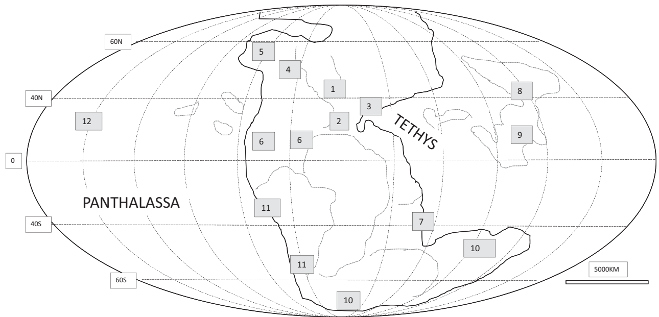
Figure 1. Global distribution of the main data sources used in this review that show evidence for humidity in the Carnian Age (or early late Triassic time in some poorly dated locations). The palaeogeographic map of Golonka (2007) is used as a template. Solid black denotes the continental shelf of Pangaea; grey lines denote supposed island masses (both continental and volcanic arc) and the shape of the continents following Mesozoic break-up and sea floor spreading. 1 – Austria, Dolomites, Hungary, Slovenia, Sicily, Spain (Dal Corso et al. 2012; Furin et al. 2006; Haas et al. 2014; Kolar-Jurkovsek & Jurkovsek, 2010; Pott, Krings & Kerp, 2008; Rostasi, Rausick & Varga, 2011); 2 – Iberia (Arche & Lopez-Gomez, 2014); 3 – Israel (Magaritz & Druckman, 1984); 4 – North Sea, Germany, UK (Kozur & Bachmann, 2010; McKie, 2014; Shukla, Bachmann & Singh, 2010; Porter & Gallois, 2008); 5 – Svalbard (Xu et al. 2014); 6 – Eastern North America (Arche & Lopez-Gomez, 2014), Utah (Prochnow et al. 2006); 7 – Indian Himalayas (Hornung, Krystyn & Brandner, 2007); 8 – China (Lehrmann et al. 2005); 9 – Indonesia (Martini et al. 2004); 10 – Australia (McLoughlin et al. 1997); 10 – Antarctica (Retallack & Alonzo-Zarza, 1998; Retallack, Veevers & Morante, 1996); 11 – Argentina (Tabor et al. 2006), Chile (Nielsen, 2005); 12 – Japan (Nakada et al. 2014).
