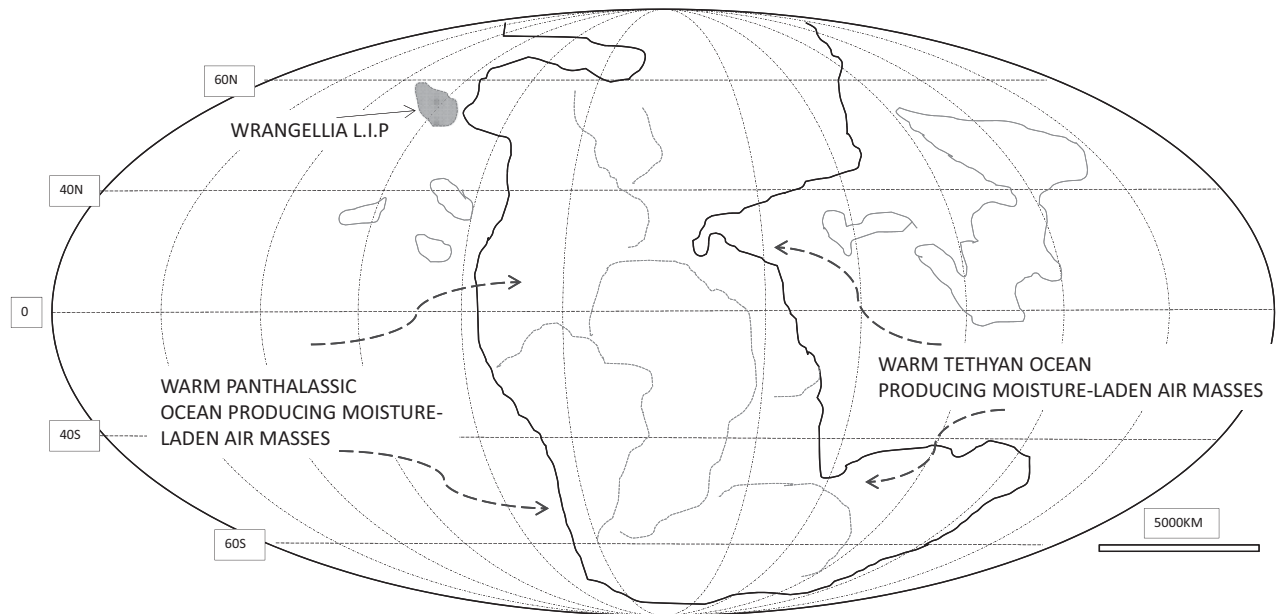
Figure 2. A model of how warming of the Carnian oceans may have increased precipitation in many (but possibly not all) of the areas studied. Palaeogeography redrawn after Golonka (2007) and possible climate scenarios after McKie (2014).
