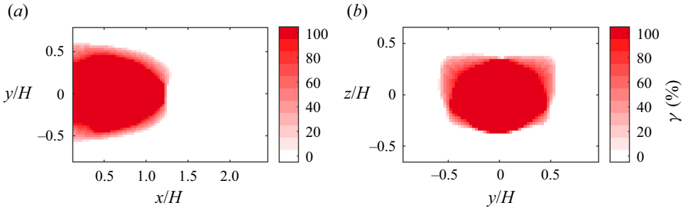
Figure 16. Backflow probabilities from U_{ROM} of the SPOD mode at St_H = 0.041 in (a) z/H = 0 and (b) x/H = 0.5 planes.
