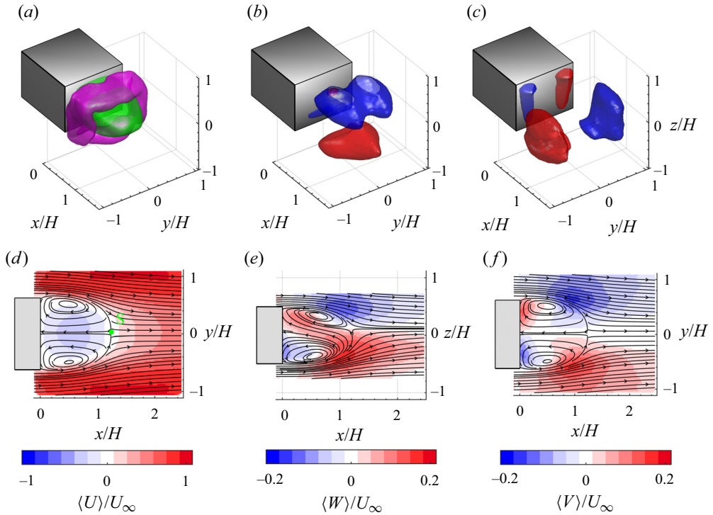
Figure 3. The 3-D and 2-D visualizations of the mean velocity field from tomo-PIV measurements. (a) Isosurface of \langle U \rangle / U_\infty = 0 (green) and normalized Q -criterion, QH^2 / U_\infty^2 = 0.48 (purple). (b) Isosurfaces of \langle W \rangle / U_\infty = \pm 0.1 , and (c) \langle V \rangle / U_\infty = \pm 0.1 . Red shows +0.1, and blue shows -0.1. (d) Two-dimensional contours of \langle U \rangle / U_\infty at z/H = 0 plane, (e) contour of \langle W \rangle / U_\infty at y/H = 0 and (f) contour of \langle V \rangle / U_\infty at z/H = 0 .
