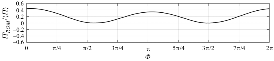
Figure 12. The normalized fluctuations of separation volume \Pi'_{ROM}/\langle\Pi\rangle based on U_{ROM} obtained using the SPOD mode at St_H = 0.007 .
