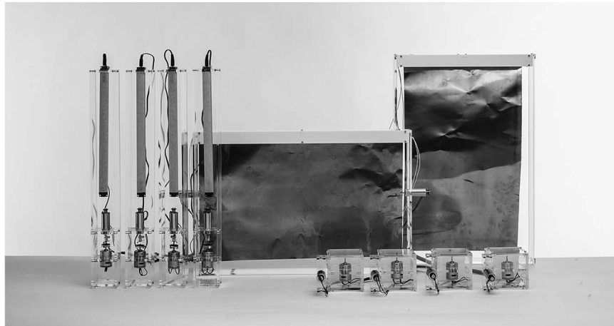
Figure 4. The Brutalist Noise Ensemble (2014) by Mo H. Zareei (left to right: Rasper \times 4, Rippler \times 2, Mutor \times 4). Photo \copyright Mo H. Zareei.
