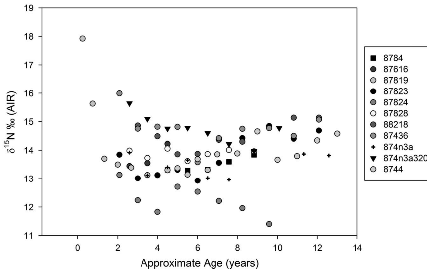
Figure 3 Childhood \delta^{15}\text{N} ratios for individuals from the cemetery of Igron VIII (Henderson 2015).
