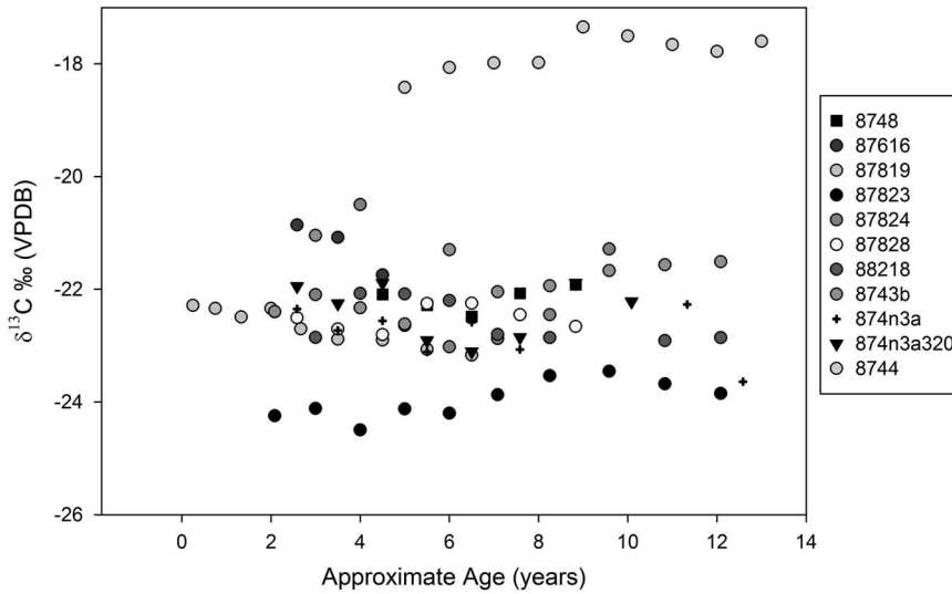
Figure 2 Childhood \delta^{13}\text{C} ratios for individuals from the cemetery of Igron VIII (Henderson 2015).
