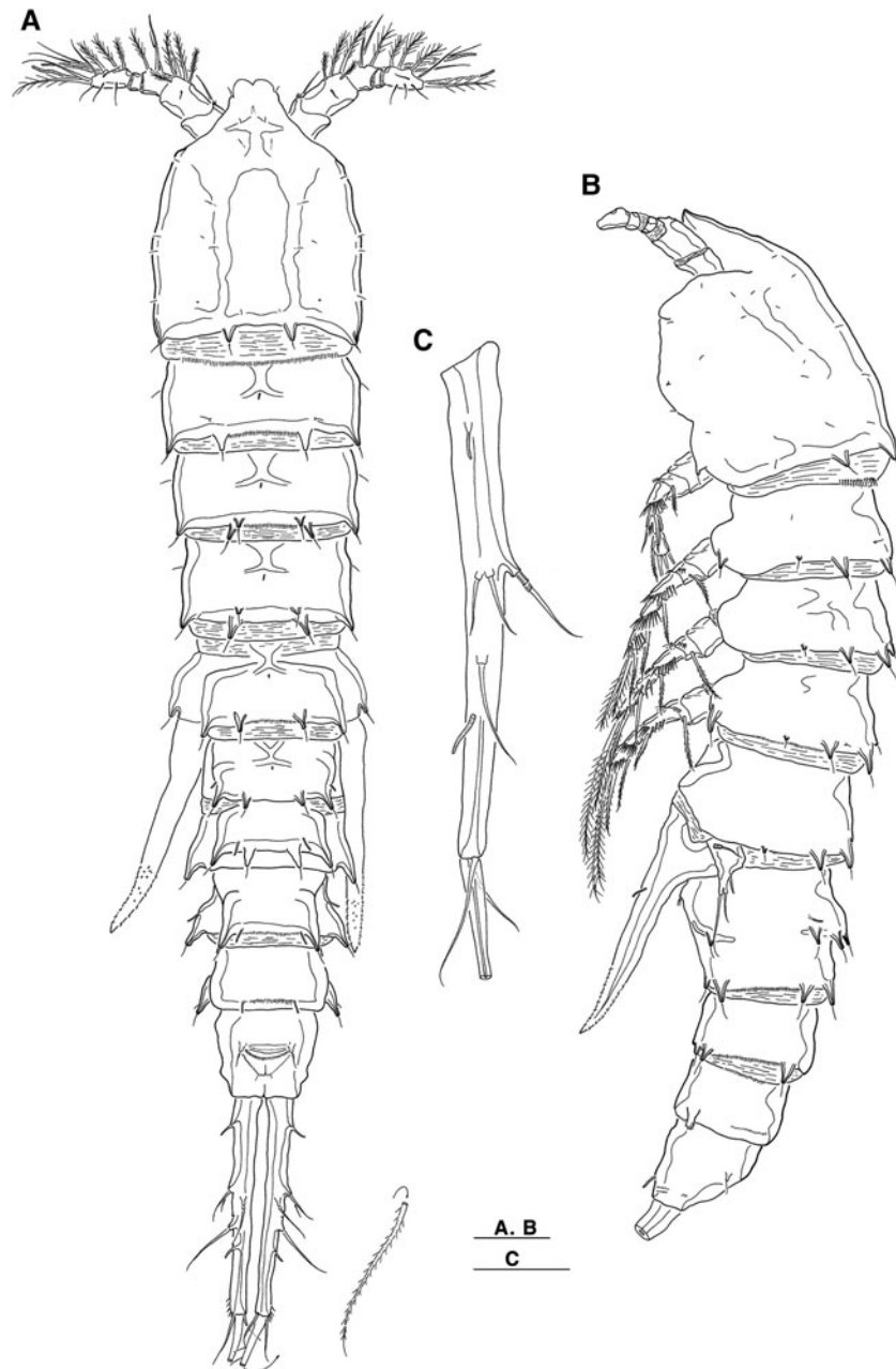
Fig. 2. Paracrenhydrosoma kiaii sp. nov., female paratype: (A) habitus, dorsal; (B) habitus, lateral; (C) left caudal ramus, lateral. Scale bars: A, B = 50 \mu\text{m} ; C = 30 \mu\text{m} .
