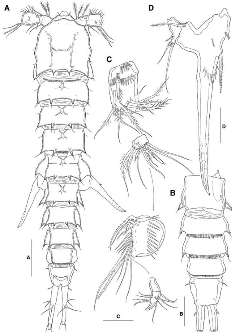
Fig. 7. Paracrenhydrosoma kiai sp. nov., male paratype: (A) habitus, dorsal; (B) urosome (excluding P5 bearing somite); (C) antennule; (D) P5. Scale bars: A, B = 50 µm; C, D = 30 µm.
