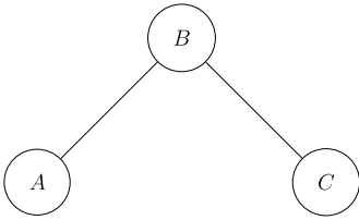
Figure 1. A graphical model with three variables and two edges.
