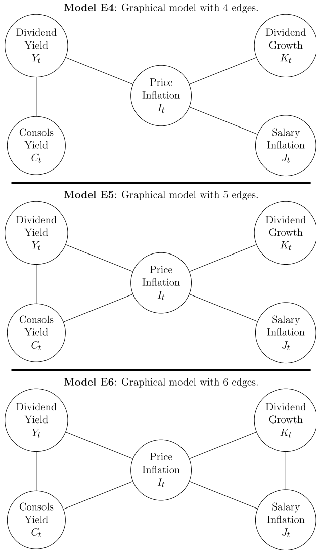
Figure 3. Optimal graphical models based on different selection criteria.
