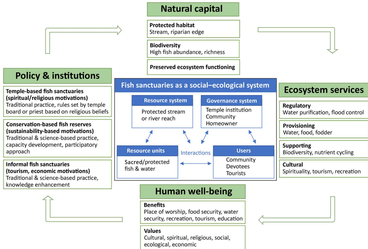
FIG. 1 Framework to characterize community-based fish sanctuaries in India as a functional social–ecological system (Table 2).
