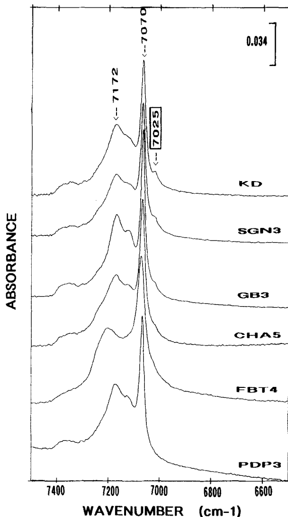
Figure 8. Diffuse reflectance NIR spectra in the 5500 – 7500\text{ cm}^{-1} region of the samples presented in Figures 4 and 6.
