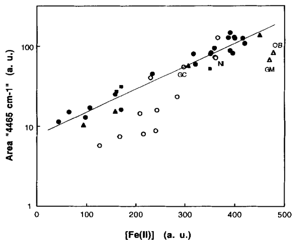
Figure 9. Semi-log plot of substituted \text{Fe}^{3+} in site II [Fe(II)] vs. area of the 4465 \text{cm}^{-1} diffuse reflectance NIR absorption band, expressed in arbitrary units (a. u.). Full circles = sedimentary kaolinites with low specific area. Full squares = hydrothermal kaolinites. Open circles = kaolinites with high specific surface area (Charentes FBT local site, and two soil samples NI and GC), with a size correction factor applied for these samples (see text). Open and full triangles = other soil kaolinites.
