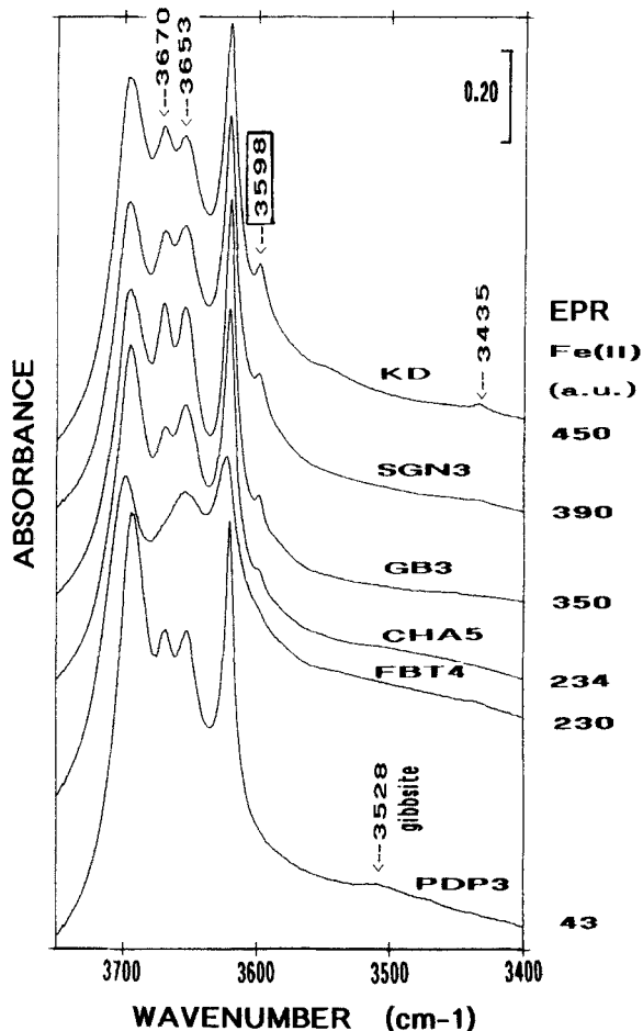
Figure 4. Diffuse reflectance IR spectra in the 3400\text{--}3750\text{ cm}^{-1} region for selected samples containing variable amounts of substituted \text{Fe}^{3+} in \text{Fe}(\text{II}) sites ( [\text{Fe}(\text{II})] , expressed in arbitrary units (a. u.).
