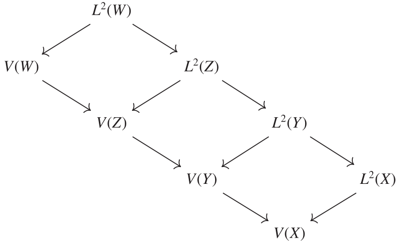
FIGURE 2. The subspace relations in Lemma 4.4.
