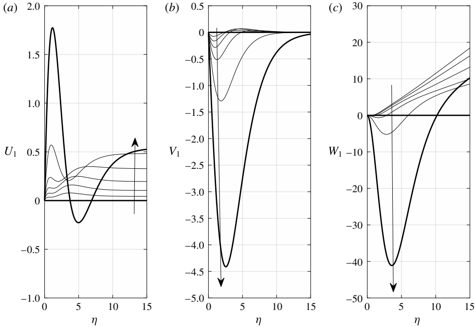
FIGURE 6. Boundary-layer velocity profiles from the numerical solution of (2.10)–(2.12) for \theta=0^\circ, 15^\circ, 30^\circ, 45^\circ, 60^\circ, 75^\circ, 80^\circ, 85^\circ according to the arrows' direction. The profiles at \theta=0^\circ and \theta=85^\circ are marked by thick lines.
