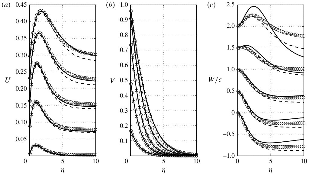
FIGURE 9. Comparison of the azimuthal (a), tangential (b) and radial (c) velocities near the sphere surface for \theta = 10^\circ, 30^\circ, 50^\circ, 70^\circ, 80^\circ and Re_s = 1500 . See figure 7 for the list of the used symbols.
