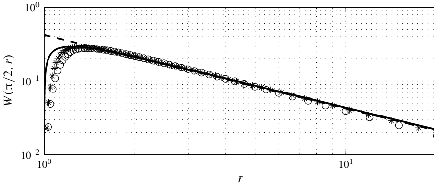
FIGURE 10. Radial velocity along the equatorial plane estimated from the numerical simulations at Re_s = 500 (O) and Re_s = 1500 (*). (—) W_j(0, r) as a solution of (2.23)–(2.26). (---) Self-similar expression (2.29).
