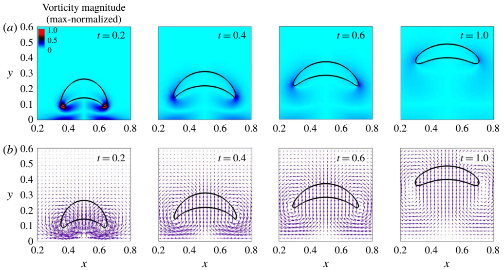
FIGURE 19. (Colour online) The maximum value of the normalized absolute vorticity (a), and the velocity vector field (b) in and around the levitating droplet. The initial horizontal location of the droplet is central in this case.
