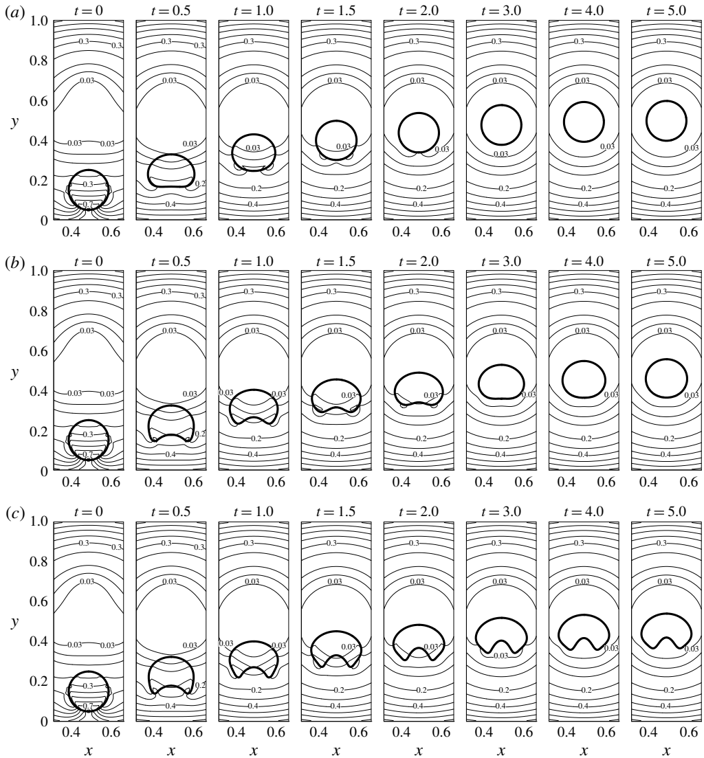
FIGURE 5. The interface of the levitating droplet and the absolute magnetic field lines for La = 10.0 (a), 1.0 (b) and 0.1 (c). Ga = 0.1 , La_m = 360 .
