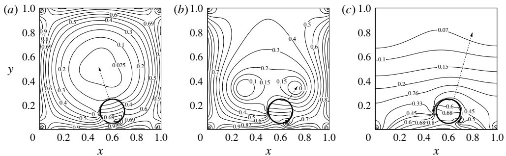
FIGURE 17. The absolute magnetic field contours around the eccentrically placed droplet when – from left to right – (a) all of the four walls are covered with alternate magnetic poles, (b) the bottom and both the side walls are covered and (c) only the bottom wall is covered.
