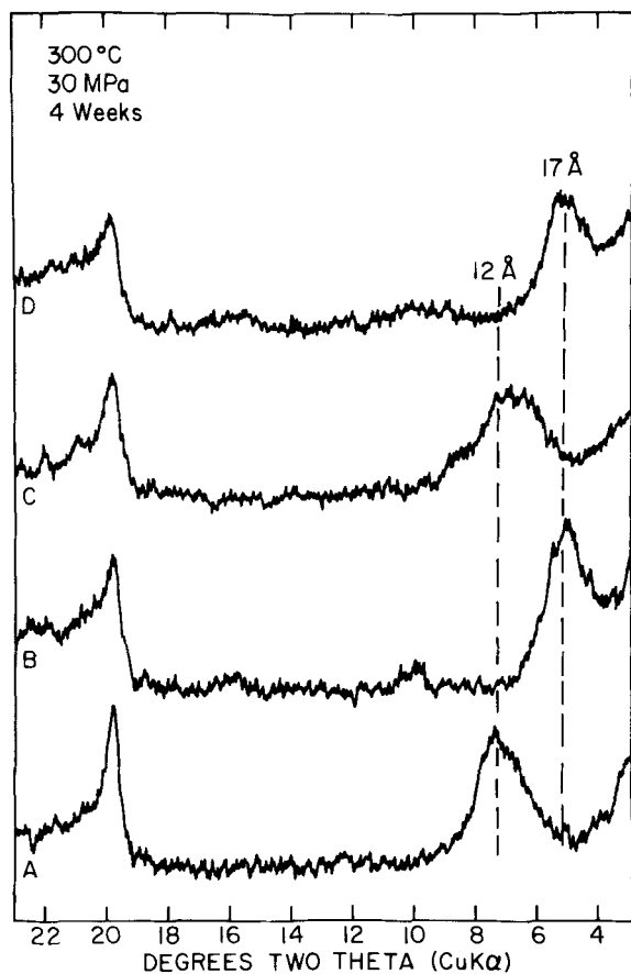
Figure 3. X-ray powder diffractograms of hydrothermal products of zeolites in Mg-rich brine. (A) 12-Å clay mineral formed from phillipsite, Pine Valley, Nevada; (B) Same as (A) but expanded to 17 Å upon exposure to ethylene glycol which indicated that it is smectite; (C) 12-Å clay mineral formed from chabazite, Christmas, Arizona; (D) Same as (C) but expanded to 17 Å upon exposure to ethylene glycol which indicated that it is smectite.
