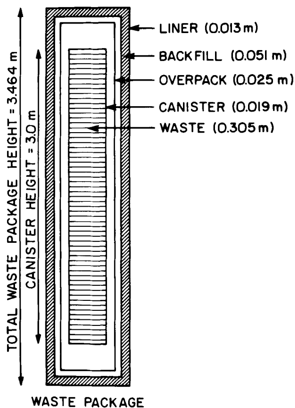
Figure 1. Waste package characteristics for commercial high level waste in a salt repository (draft interim reference repository conditions for commercial and defense high-level nuclear waste and spent fuel repositories in salt by The Reference Repository Conditions Interface Working Group, NWTs-3, September 1981). According to the current designs, backfill for salt waste packages is a backup option.
