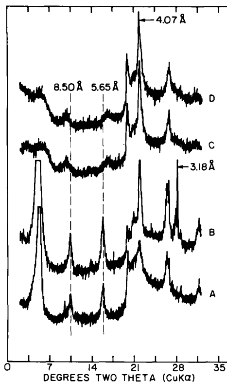
Figure 2. X-ray powder diffractograms of montmorillonite from Texas. (A) Ethylene glycolated; (B) Hydrothermally treated at 300°C/30 MPa/4 weeks in NaCl brine showing albite (3.18 Å); (C) Hydrothermally treated at 300°C/30 MPa/4 weeks in Mg-rich brine showing randomly interstratified montmorillonite/illite; (D) Same as (C) but after 12 weeks.
