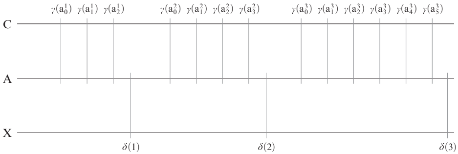
FIGURE 4. G(1) = \{a_0^1, a_1^1, a_2^1\} , etc.
