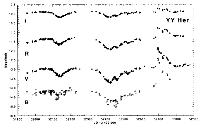
Fig. 1. BVR photometry of YY Her secured during international campaign from 2001 to 2003.
