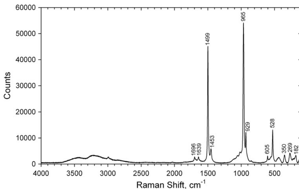
Fig. 3. Raman spectrum of davidbrownite-(NH 4 ).
