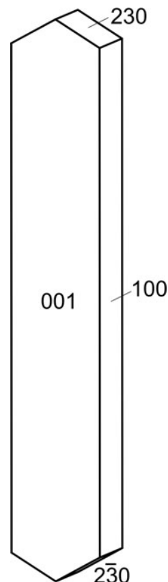
Fig. 2. Crystal drawing of davidbrowneite-(NH 4 ); clinographic projection in a non-standard orientation, \mathbf{b} vertical.
