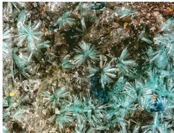
Fig. 1. Sprays of davidbrowneite-(NH 4 ) needles with deep blue antipinite on quartz-baryte matrix; Field of view 1.14 mm. Specimen number 66951.
