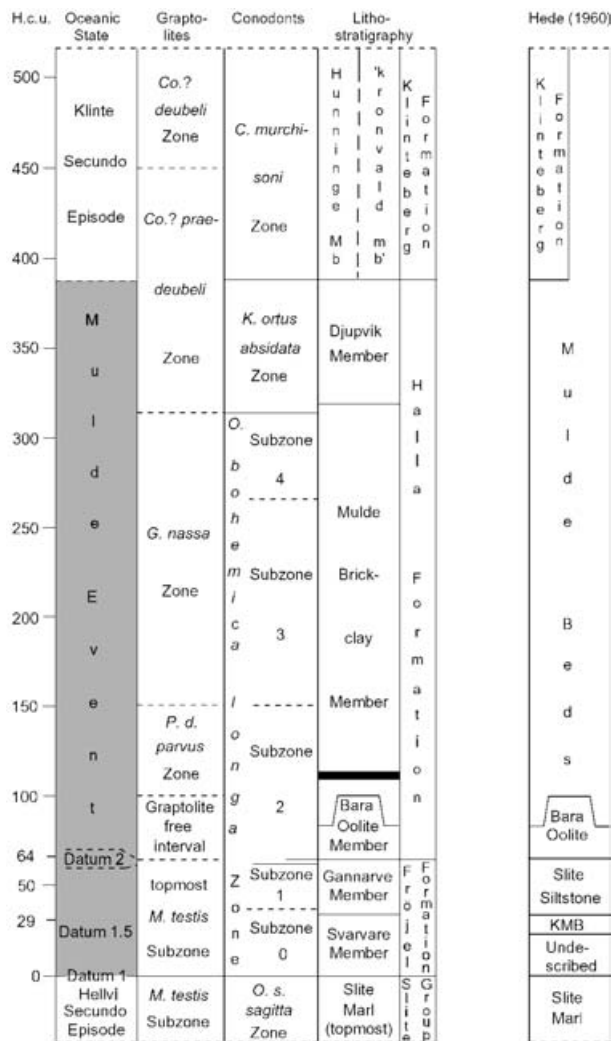
Figure 2. Revised stratigraphic framework of the Late Wenlock of Gotland. The left margin shows the Homerian chonal unit scale (H.c.u.) of Jeppsson & Calner (2003). The right column shows the subdivision of Hede (1960). KMB is an abbreviation for 'Kalksandstenens Märgliga Bottenlager' (Hede, 1917; 'the marly bottom layer of the carbonate sandstone'). The black bar in Subzone 2 of the O. b. longa Zone indicates the stratigraphic position of the Grötlingbo Bentonite. This is a 0.10–0.38 m thick, basin-regional marker, identified in the När-1, Grötlingbo-1, Ohsaare, and Priekule drillcores. Extensive silicification below it forms indirect evidence for its presence on western Gotland.
