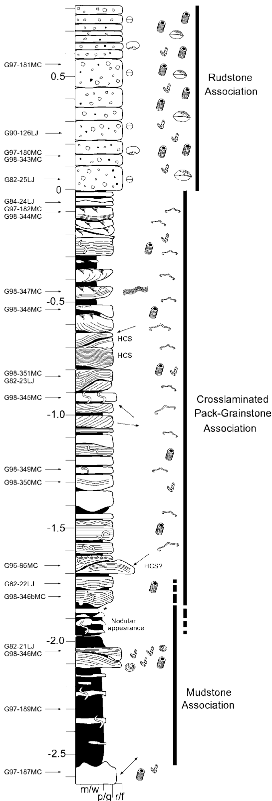
Figure 9. Sedimentary profile showing the Loggarve 2 roadcut. The three subdivisions represent, from the bottom, the Mulde, Djupvik, and the Hunninge members. Facies are interpreted as reflecting progradation of crinoid shoal facies across a storm-dominated, proximal platform slope. The asterisk indicates a distinct horizon useful as an ancillary reference level, 1.80–1.88 m below the boundary [‘plastic clay’ of Jeppsson & Jerre (unpublished)]. See also photographs in Fig. 8b,c.
