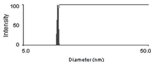
Fig. 2. A typical particle size distribution measurement by dynamic light scattering.
