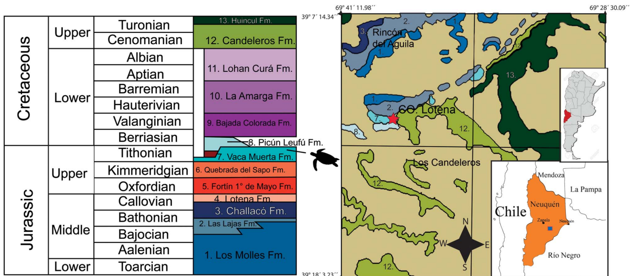
Figure 1. Stratigraphic column and map showing outcrops of Vaca Muerta Formation at Cerro Lotena locality where Neusticemys neuquina was found. Picun Leufu geologic map modified from Leanza and Hugo (1997). The star represents the location where MOZ-PV-064 was discovered and the turtle outline in the stratigraphic column represents the stratigraphic provenance of MOZ-PV-064.
