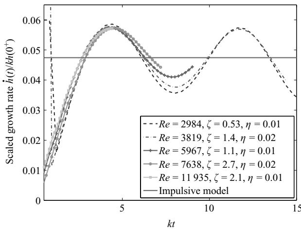
FIGURE 10. Plots of perturbation amplitude growth rate \dot{h}(t)/kh(0^+) against dimensionless scaled time kt , for the case M_I = 1.21 , A = 0.2 . Both Reynolds number and interface wavelength to thickness ratio \eta vary in this case.
