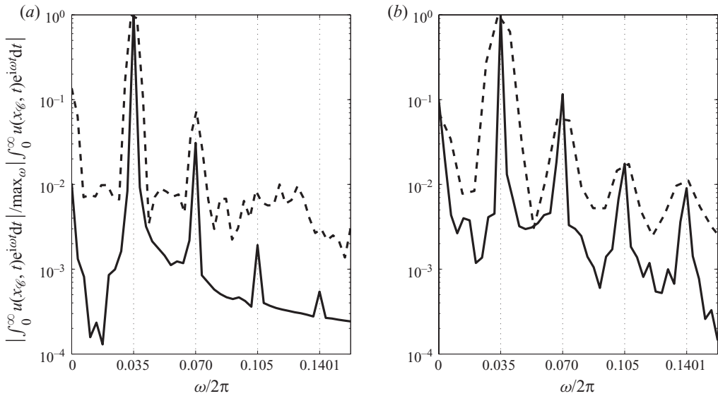
FIGURE 10. Vertically averaged temporal Fourier spectra of horizontal velocity normalized by their maximum amplitude. The data were obtained from cuts at x_{\phi} = 0.075 m for (a) A_0 = 0.005 m and (b) A_0 = 0.035 m, for experiments (---) and numerics (—).
