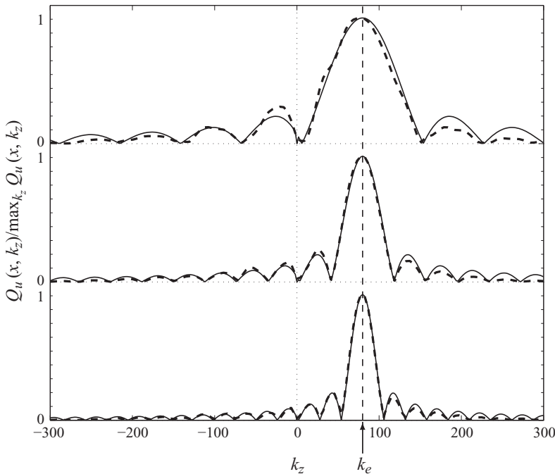
FIGURE 7. Comparison between spatial spectra Q_u(x, k_z) computed from the experiments (---) at station x_\phi = 0.05 m and the theoretical expression (—) computed from (3.4) on the boundary x = 0 , for W = \lambda_e (top), W = 2\lambda_e (middle) and W = 3\lambda_e (bottom).
