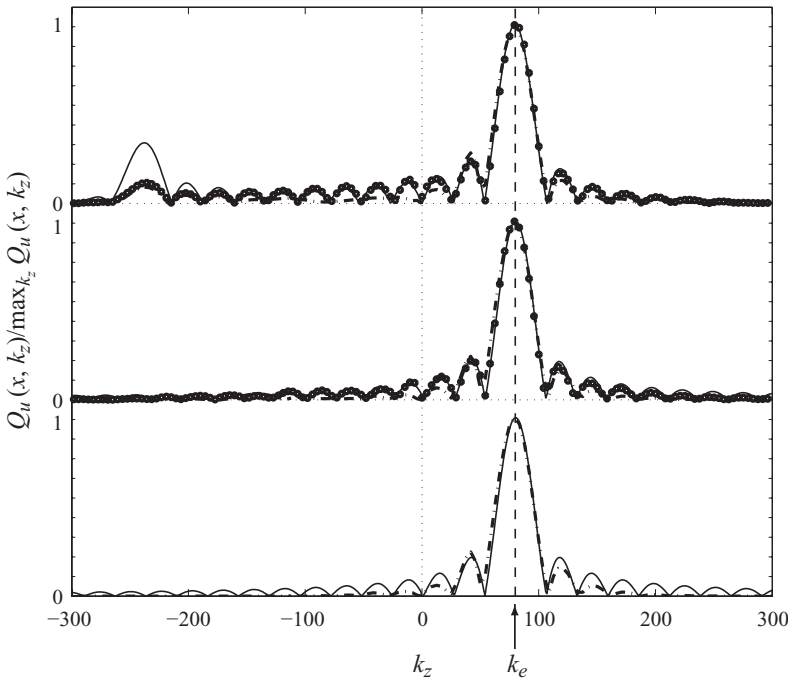
FIGURE 9. Comparison between spatial spectra Q_u(x, k_z) computed from the experiments ( \circ ) and numerical simulations ( -\cdot-\cdot- ) at station x_{\mathcal{C}} = 0.05 m and the theoretical expression (—) computed from (3.4) on the boundary x = 0 , for M = 4 (top), M = 12 (middle) and M = \infty (bottom).
