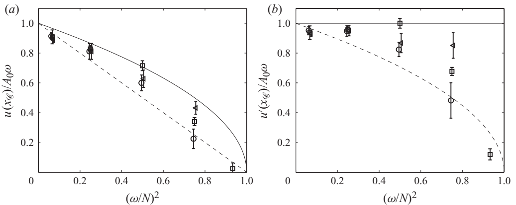
FIGURE 5. Comparison of numerical results ( \square ) and experimental results for the vertical ( \circ ) and tilted ( \triangleleft ) wave generators for the mean amplitude and standard deviation of (a) u/A_0\omega and (b) u'/A_0\omega . Results are plotted as a function of (\omega/N)^2 for different frequencies corresponding to \theta = 15^\circ, 30^\circ, 45^\circ, 60^\circ and 75^\circ (numerics only). The solid lines correspond to u'/(A_0\omega) = 1 and the dashed lines to u'/(A_0\omega) = \cos\theta .
