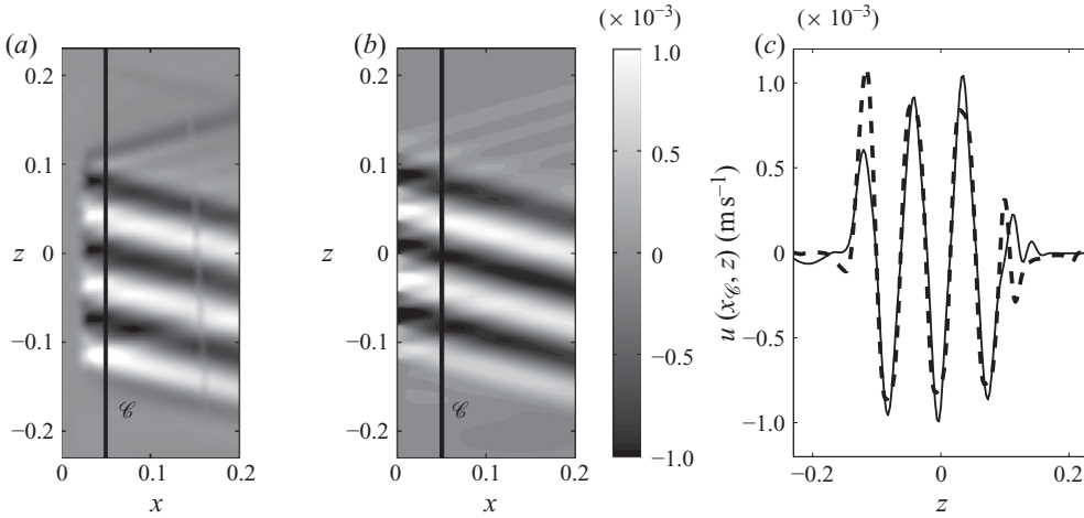
FIGURE 8. Horizontal velocity fields for (a) experiment and (b) simulation for case 12 in table 2 with M = 4 . (c) Vertical profiles along the cut \mathcal{C} located at x_{\mathcal{C}} = 0.05 m for the experiment (---) and the simulation (—). All lengths are in metres and all velocities in metres per second.
