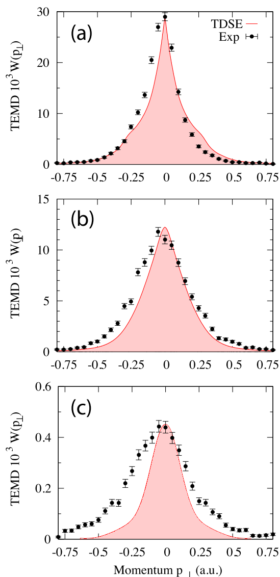
Figure 24. Figure adapted from Ivanov et al. [114] . TEMD of Ar for (a) \varepsilon = 0 , (b) \varepsilon = 0.42 and (c) \varepsilon = 1 , respectively. The peak laser intensity is measured to be (4.8 \pm 2.4) \times 10^{14} \text{ W cm}^{-2} . Theoretical data is shown as the red curve, experimental data is plotted.
