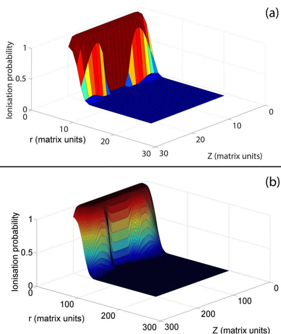
Figure 12. The modelling of the 2D ionization fraction map with the following laser parameters: I_{pk} = 9.6 \times 10^{13} \text{ W cm}^{-2} ; w_0 = 7.25 \mu\text{m} ; pulse length = 6.3 fs. (a) Shows the calculated points, while (b) shows the interpolated map. Both maps come from the same modelling data; however, only the interpolated map was used for further processing.
