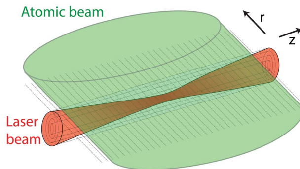
Figure 11. A conceptual layout of the interaction region as it was modelled for theoretical ion yield predictions.
