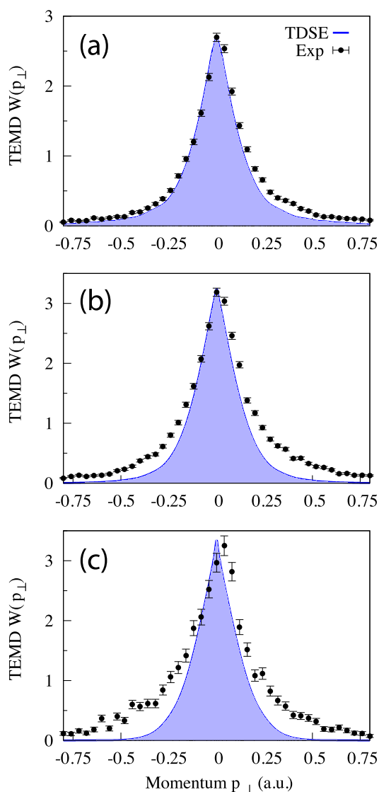
Figure 25. Figure adapted from Ivanov et al. [114] . TEMD of Ne* for (a) \varepsilon = 0 , (b) \varepsilon = 0.42 and (c) \varepsilon = 1 , respectively. The peak laser intensity is measured to be (2.0 \pm 1.0) \times 10^{14} \text{ W cm}^{-2} . Theoretical data is shown as the blue curve, experimental data is plotted.
