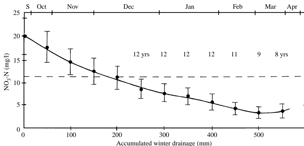
Fig 3. Mean concentration of \text{NO}_3\text{-N} (mg/l) in winter drainage from the grazed grass pasture receiving 200 kg N/ha per annum. Based on the 13-year period 1983–95 unless otherwise indicated. The EU limit in drinking water is also indicated (---). Vertical bars represent s.e.s.
