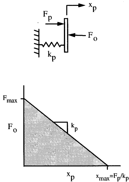
Fig. 11. (top) Quasi-static model of PZT stack actuator and (bottom) region of attainable output (region of operation).
