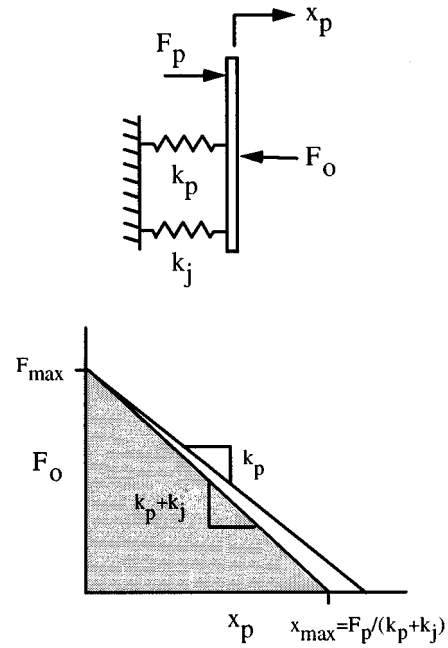
Fig. 12. (top) Quasi-static model of PZT with compliant mechanism joint stiffness and (bottom) region of attainable output (region of operation).
