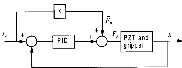
Fig. 4. PZT-actuated compliant mechanism position controller. The feed-forward term is a simple quasi-static model of the PZT and compliant mechanism (i.e., a pure stiffness), which provides a command estimate for the desired position, and the PID loop provides correction of the estimate for model error.
