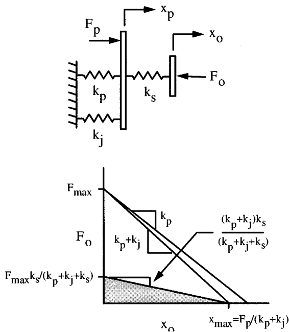
Fig. 13. (top) Quasi-static model of PZT with compliant mechanism joint stiffness and structural compliance and (bottom) region of attainable output (region of operation).
