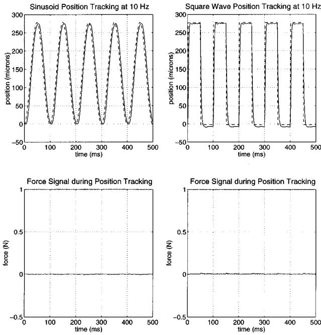
Fig. 6. Closed-loop time domain behavior of position control loop for a 10 Hz sinusoid (left column) and square wave (right column), showing the desired (dashed) and the actual (solid) position, and the corresponding force sensor signals (illustrating sensor decoupling).
