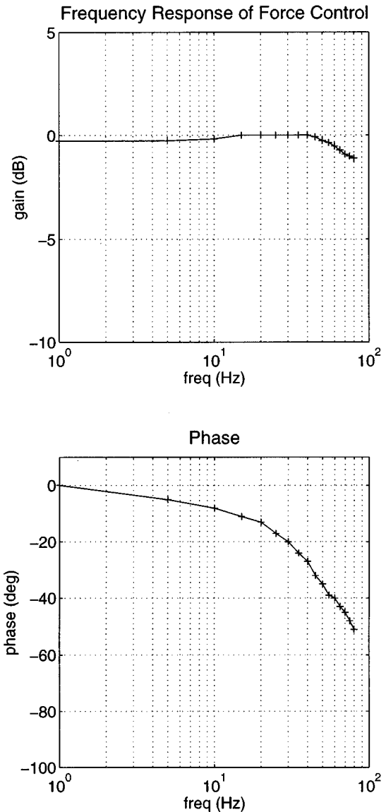
Fig. 8. Frequency response of force control loop. Data was acquired at a 5 kHz controller sampling rate.
