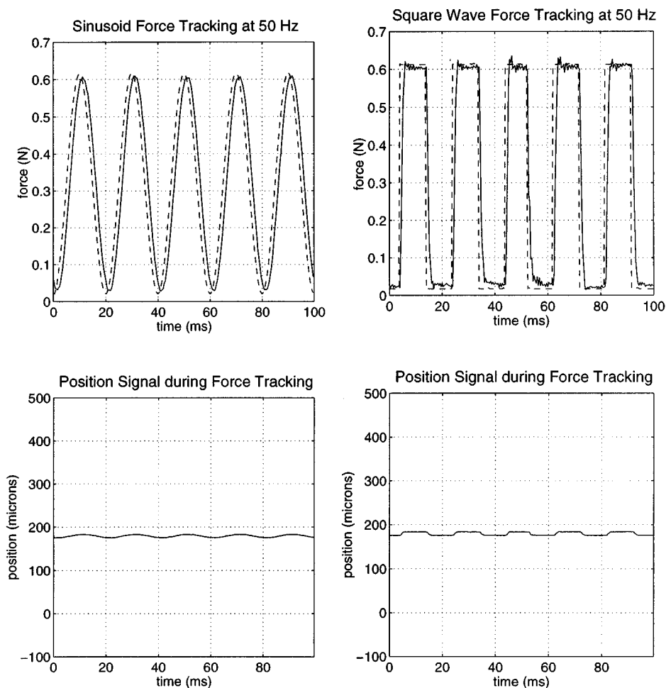
Fig. 9. Closed-loop time domain behavior of force control loop for a 50 Hz sinusoid (left column) and square wave (right column), showing the desired (dashed) and the actual (solid) force, and the corresponding position sensor signals (illustrating sensor decoupling). Note that the fluctuations in the position signal are due to compliance of the object and limited stiffness of the gripper structure, rather than fundamental sensor coupling.
