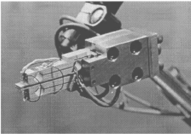
Fig. 3. Instrumented microgripper prototype.
