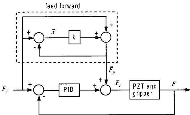
Fig. 7. PZT-actuated compliant mechanism force controller. The feed-forward term is a simple quasi-static model of the PZT and compliant mechanism (i.e., a pure stiffness) that includes a state estimator for estimating position. The feed-forward model provides a command estimate for the desired position, and the PID loop provides correction of the estimate for model error.
