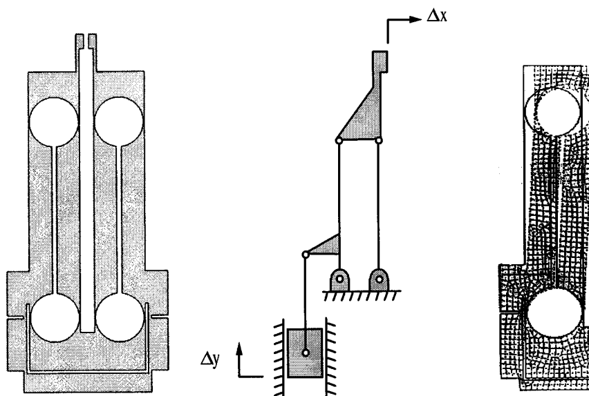
Fig. 2. (left) Two-dimensional drawing of microgripper structure, (middle) idealized schematic of (one half of) flexure-based linkage, and (right) finite element analysis illustrating motion of (one half of) gripper.
