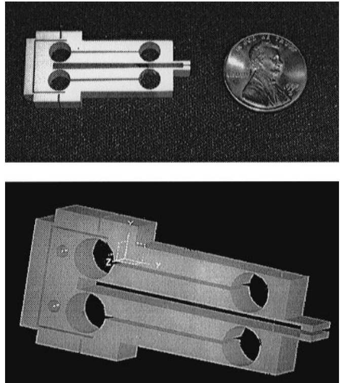
Fig. 1. (top) Flexure-based microgripper structure and transmission and (bottom) solid model of gripper design.
