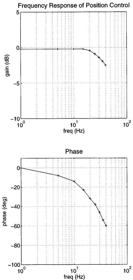
Fig. 5. Frequency response of position control loop. Data was acquired at a 5 kHz controller sampling rate.
