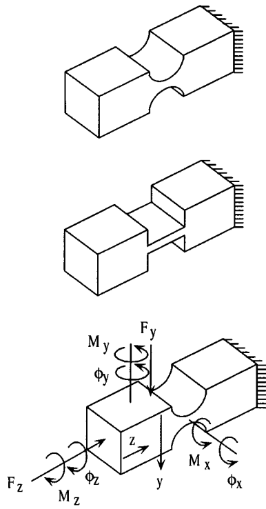
Fig. 10. (top) Typical flexure geometry, (middle) thin, flat flexure geometry, such as the super-elastic flexure of Horie et al., and (bottom) loading diagram illustrating the stiffness along the direction of rotation and compliance in all other directions.
