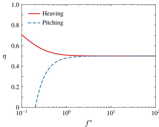
FIGURE 5. (Colour online) Efficiency as a function of reduced frequency f^* for a heaving (red) and pitching (blue) rigid plate. At low f^* , a pitching rigid plate produces drag in the mean, hence its efficiency is negative.
