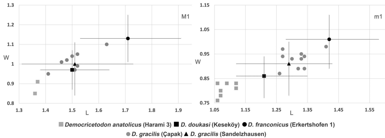
Figure 5. Scatter diagram of the upper and lower first molars of small sized Democricetodon from Anatolia and adjacent area (data are after Klein Hofmeijer and De Bruijn, 1988; Theocharopoulos, 2000; Wessels and Reumer, 2009).
