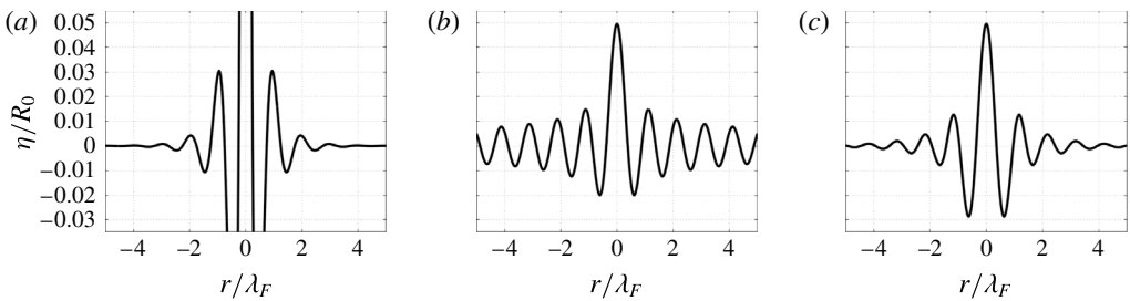
FIGURE 8. Different model predictions of the free-surface cross-section of a (2, 1)^1 bouncer at the moment before impact with \Gamma = 3.1 . (a) The cosine wave model (3.9) of Eddi et al. (2011) with a spatial damping with decay length 1.6\lambda_F reported by the authors. Note the singularity at r = 0 . (b) The Bessel model (3.10) of Moláčěk & Bush (2013b). (c) The result of our computation.
