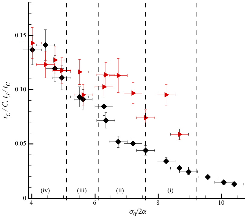
Figure 23. Maximum cavity thickness, t_C/C (◆), and re-entrant flow thickness, t_J/t_C (red triangle right), varying with \sigma_0/2\alpha .
