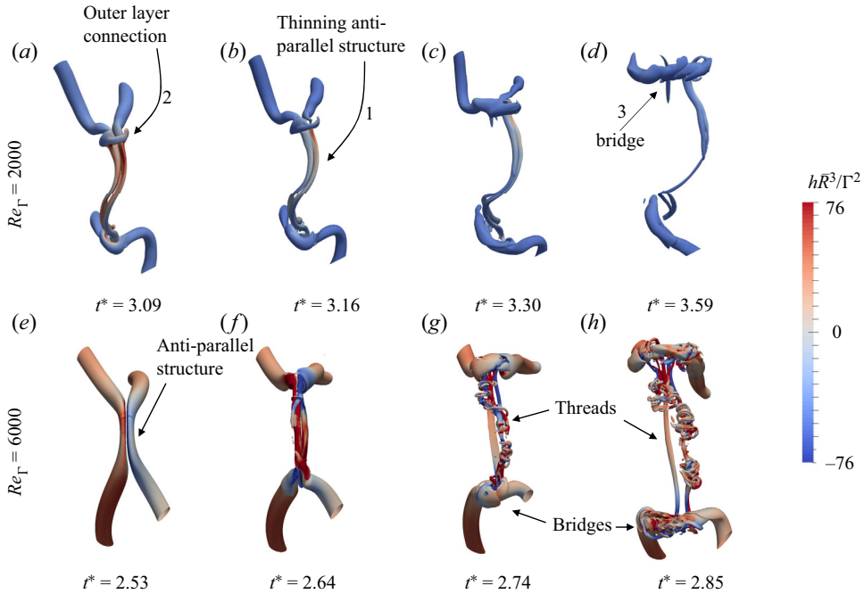
FIGURE 13. Visualization of the generation of hairpin vortices from Q -isosurfaces at QR^4/\Gamma^2 = 96 for Re_\Gamma = 2000 and Re_\Gamma = 6000 from DNS/AMR data, coloured by normalized helicity density; threads created during the bridging process, intermediate hairpin vortex structure the final dominant hairpin structure are illustrated.
