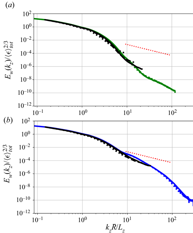
FIGURE 5. Grid sensitivity analysis for Cartesian CvP-LES (black) and AMR (green/blue) simulations: Re_\Gamma = 2000 (a), Re_\Gamma = 6000 (b) showing the one-dimensional energy spectra in the z direction at the time of first reconnection ( t_1 ) defined as the time when the maximum dissipation is achieved (see figure 2). Grid resolutions considered are the finest three datasets from each simulation: coarse ( \cdots ); intermediate ( -\ - - ); fine ( — ) (see data in table 2). Red dotted line shows a reference -5/3 slope. Here L_z is the domain size in z direction.
