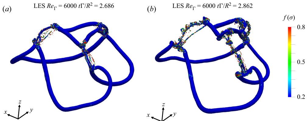
FIGURE 12. Sensor function f(\sigma) used in the CvP-LES closure in (2.16) at two different time instances from a LES at Re_\Gamma = 6000 .
