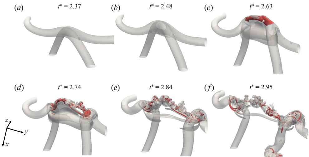
FIGURE 15. Isosurfaces of vorticity magnitude at specific time steps during reconnection: \omega = 0.5\Gamma/\pi r_{e,0}^2 coloured in transparent grey and \omega = 3.0\Gamma/\pi r_{e,0}^2 coloured by red at Re_\Gamma = 6000 .
