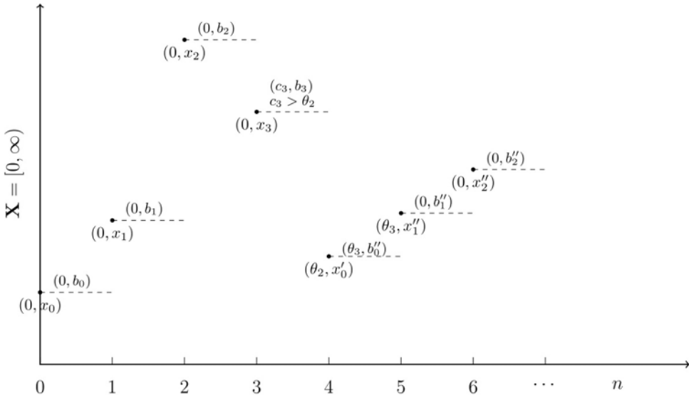
FIGURE 2: The realization of the state process in the hat DTMDP model corresponding to the sample path in the gradual-impulse control problem in Figure 1. The time index is discrete from \{0, 1, \dots\} . The realizations of the components \{(C_n, B_n)\}_{n=0}^\infty in the action process \{\hat{A}_n\}_{n=0}^\infty are indicated above the dashed lines between consecutive states. For example, (0, b_0) next to the state (0, x_0) indicates that the decision-maker applies an impulse b_0 immediately, which results in the next state (0, x_1) . All the components x_0, x_1, \dots, x'_0, x'_1, x'_2 and b_1, b_2, b'_0, b'_1, b'_2 are the same as in Figure 1. The only exception is (c_3, b_3) , which does not appear in Figure 1. Nevertheless, c_3 > \theta_2 , because in Figure 1, the first jump in the marked point process therein at the time moment \theta_1 + \theta_2 = \theta_2 is triggered by a natural jump.
