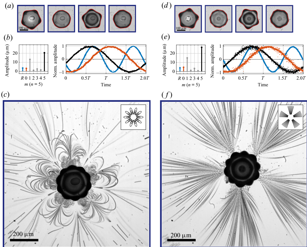
Figure 16. Modal analysis of the dynamics and associated microstreaming pattern of a microbubble of equilibrium radius 112.1 \mu\text{m} oscillating on a sectoral mode and a zonal mode of degree n = 5 , generating a 2n -lobe flower-shaped streaming pattern (a–c) and of a microbubble of equilibrium radius 110.2 \mu\text{m} oscillating on a sectoral mode and a zonal mode of degree n = 5 , generating an n -pointed star-shaped streaming pattern (d–f). The information is structured similarly to that in figure 4.
