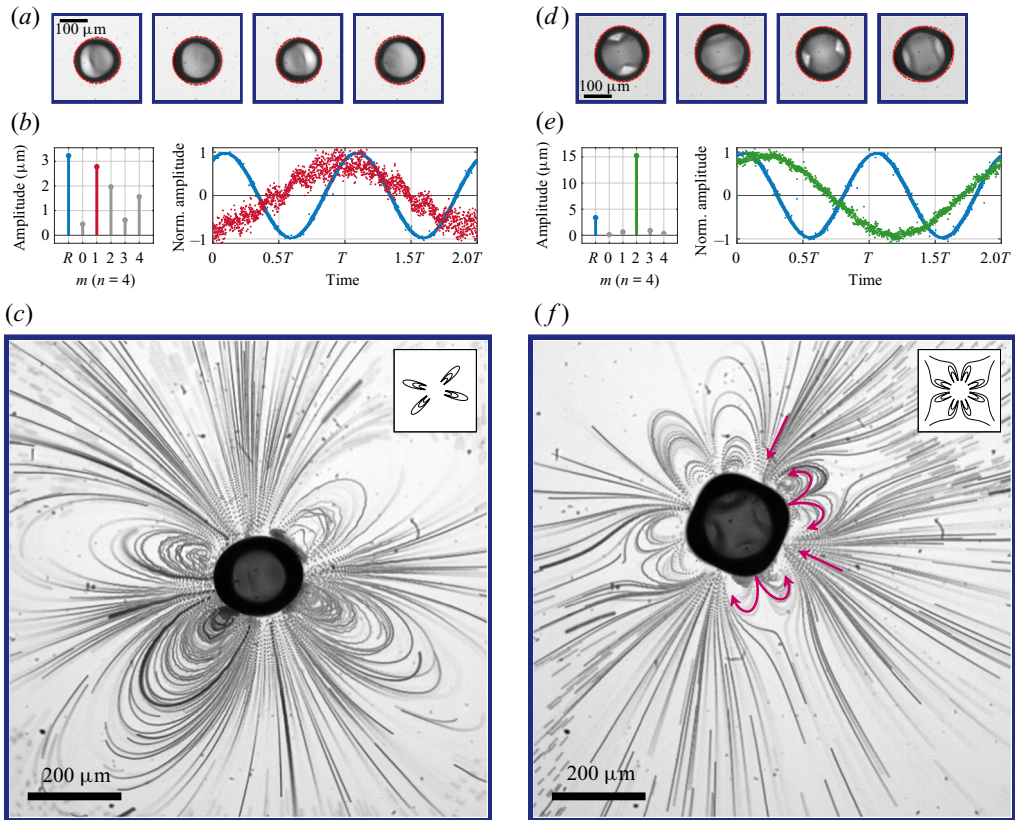
Figure 10. Modal analysis of the dynamics and associated microstreaming pattern of a microbubble of equilibrium radius 86.4\ \mu\text{m} oscillating on a tesseral mode of order m = 1 (a–c) and a microbubble of equilibrium radius 102.6\ \mu\text{m} oscillating on a tesseral mode of order m = 2 (d–f). Both are generating a 4m -lobe flower-shaped pattern. The information is structured similarly to that in figure 4.
