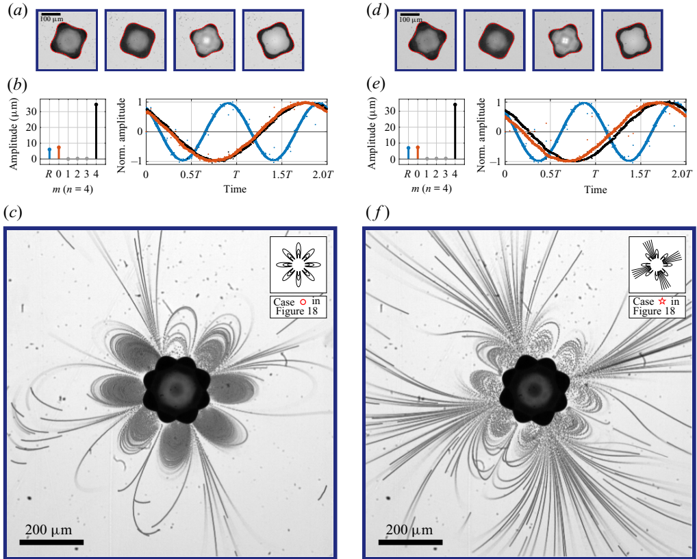
Figure 17. Modal analysis of the dynamics and associated microstreaming pattern of a microbubble of equilibrium radius 87.4 \mu\text{m} oscillating on a sectoral and a zonal mode of degree n = 4 generating a 2n -lobe flower-shaped streaming pattern (a–c) and of a microbubble of equilibrium radius 87.7 \mu\text{m} oscillating on a sectoral and a zonal mode of degree n = 4 generating a 2n -lobe flower-shaped streaming pattern accompanied by the early stages of a star shape (d–f). The information is structured similarly to that in figure 4.
