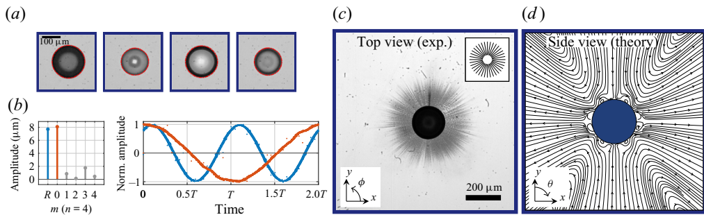
Figure 4. Modal analysis and associated microstreaming pattern of a microbubble of equilibrium radius 84.3 \mu\text{m} oscillating on a zonal mode of degree n = 4 . The information is structured as follows. (a) Snapshot series of the top-view contour display the microbubble at different instants along a complete subharmonic period of duration 2/f_0 . The red contour is a numerical reconstruction issued from the processed modal amplitudes displayed in (b). (b) Left: spectrum of the excited modes n = 4 , ‘R’ standing for the amplitude of the radial (volumetric) oscillation R(t) as defined in (3.1). Right: temporal evolution of the normalized (norm.) amplitudes of the predominant radial and zonal oscillations. (c) The associated microstreaming pattern. (d) Theoretical prediction of the side-view microstreaming induced by the self-interaction of a zonal axisymmetric mode of degree n = 4 , issued by Inserra et al. (2020a).
