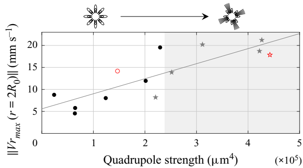
Figure 18. The preferential appearance of flower shapes ( \bullet ) or flower shapes with early stages of star shapes ( \star ) induced by a combination of sectoral and zonal modes of degree n = 4 is investigated as a function of their quadrupole strength = a_{40}a_{44}R_0^2 \sin \Delta\Phi correlated by the maximal velocity of propelled particles Vr_{max} measured at a distance r = 2R_0 from the bubble barycentre, for which a linear regression is drawn in grey. Two particular red open markers represent the two cases selected in figure 17 and their positions in this quadrupole strength map.
