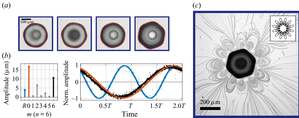
Figure 19. Modal analysis of the dynamics and associated microstreaming pattern of a microbubble of equilibrium radius 135.8\ \mu\text{m} oscillating on a sectoral mode and a zonal mode of degree n = 6 , generating a 2n -lobe flower-shaped pattern. The information is structured similarly to that in figure 4 .
