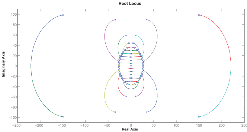
FIGURE 1. Root locus for 1 + \gamma^2 G(s)G(-s) = 0 when \sigma = 0.8 .
