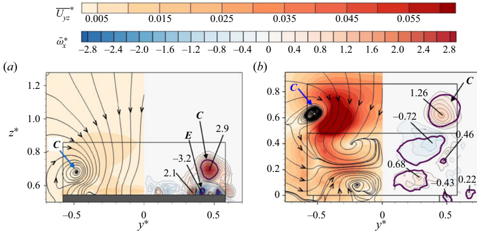
Figure 15. Time-averaged streamlines, superimposed with the \overline{U}_{yz}^* contours, and \overline{w}_x^* -contours in the (y, z) planes of (a) x^* = -0.09 and (b) 0.43 under the optimized combination of actuations, where the thick purple closed contours correspond to the time-averaged swirling strength \overline{\lambda_{ci}^2} = 0.001 .
