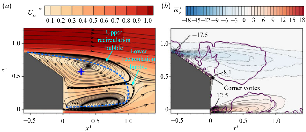
Figure 20. Time-averaged streamlines (a) superimposed with the \overline{U_{xz}}^* -contours, and the \overline{\omega}_y^* -contours (b) in the (x, z) plane of y^* = 0 under BR_e . The blue symbol '+' in (a) denotes the focus and the thick blue broken line indicates the bubble size in the unforced flow determined from the streamlines in figure 5(a); the thick purple closed contours in (b) correspond to the time-averaged swirling strength \overline{\lambda_{ci}^2}^* = 0.1 .
