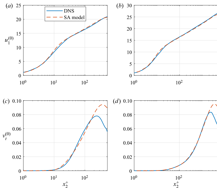
Figure 3. (a,b) Profiles of streamwise velocity (b,d) and of the turbulent eddy viscosity in plane channel from the SA model (— — —) and from the direct numerical simulation (DNS) (—) of Lee & Moser (2015). Data is shown for Re_\tau = 550 in panels (a,c) and Re_\tau = 5200 in panels (b,d).
