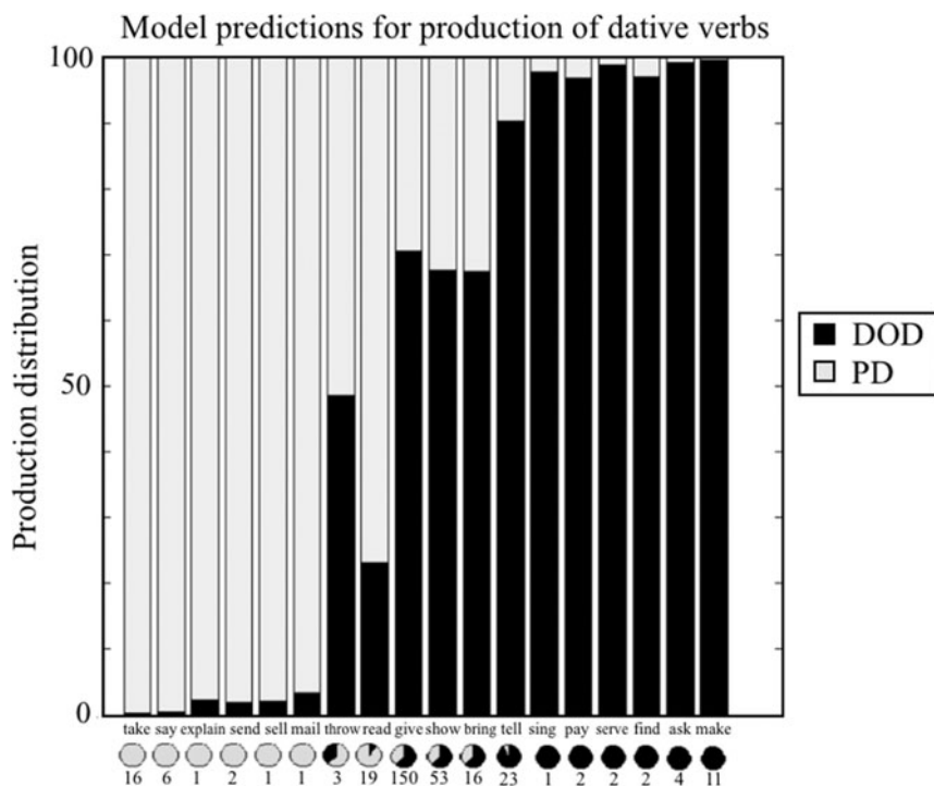
Fig. 4. Production predictions of Model K-L 3 for each verb in the full corpus. High-frequency verbs' constructions are produced at a distribution close to their empirical distribution, while low-frequency verbs are more likely to be overgeneralized (produced in a construction that they did not occur in in the input). The production distribution is denoted with the stacked bars; the associated pie chart depicts each verb's observed distribution, and its empirical frequency is the number under the pie chart.
