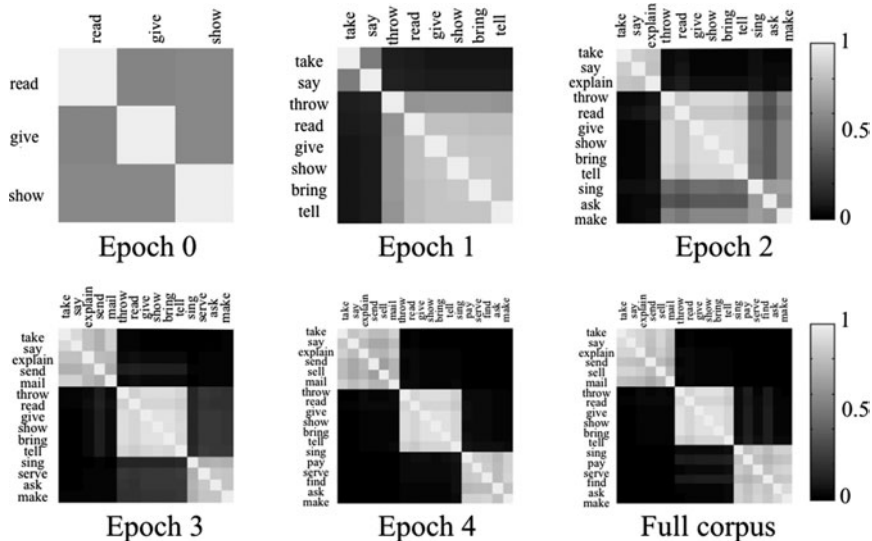
Fig. 3. Class assignments given by Model K-L3. Lighter colors indicate increasing probability that the verbs in that row and column are assigned to the same class. The diagonal is always white because each verb is always in the same class as itself.
