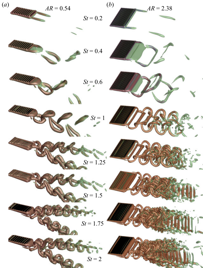
Figure 3. Influence of St on the wake vortex topology past a rigid pitching panel for AR = 0.54 and AR = 2.38 . All 3-D perspective views of the vortical structures are visualised by plotting Q -criterion with Q = 1 . Note, all the instantaneous Q -criterion structures are shown at the same dimensionless instant.
