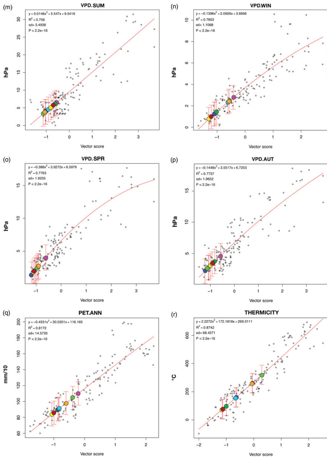
Fig. 8. CLAMP regression models for the WorldClim2_3brc modern vegetation calibration sites (open black circles) and predicted climate variables for eight early Late Cretaceous fossil sites (coloured circles as in the key shown in Fig. 6b). VPD.SUM – mean summer vapour pressure deficit, VPD.WIN – mean winter vapour pressure deficit, VPD.SPR – mean spring vapour pressure deficit, VPD.AUT – mean autumn vapour pressure deficit.
