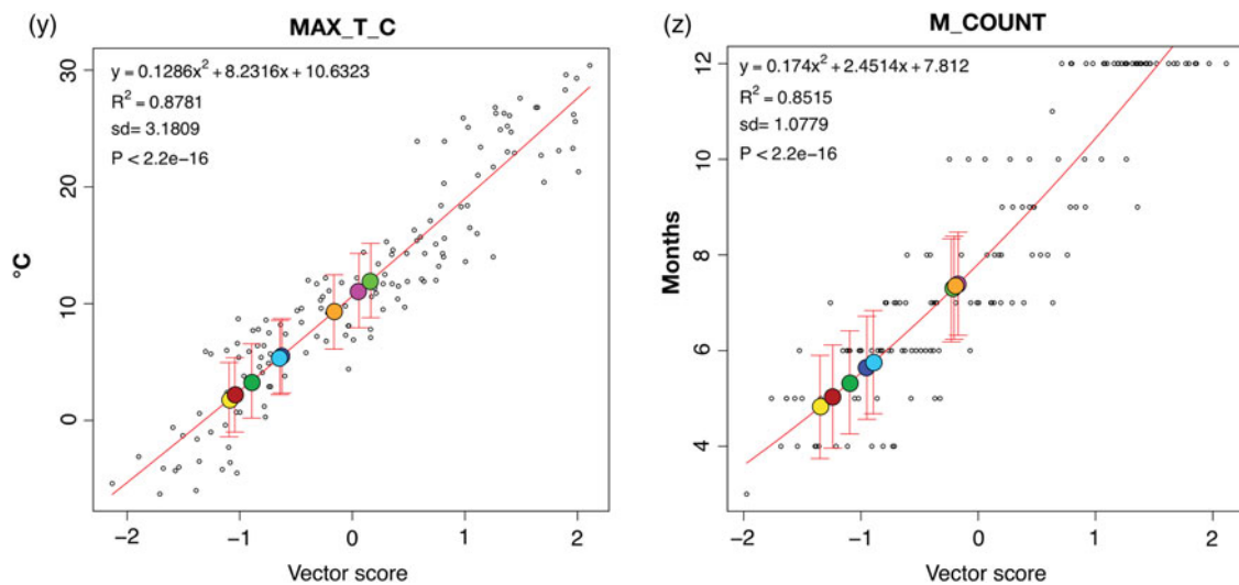
Fig. 10. CLAMP regression models for the WorldClim2_3brc modern vegetation calibration sites (open black circles) and predicted climate variables for eight early Late Cretaceous fossil sites (coloured circles as in the key shown in Fig. 6b). MAX_T_C – maximum temperature during the coldest month; M_COUNT – number of months where the temperature is above +10 °C.
