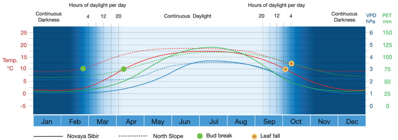
Fig. 3. Light, thermal and humidity regime for fossil assemblages at palaeolatitude ~80° N.
