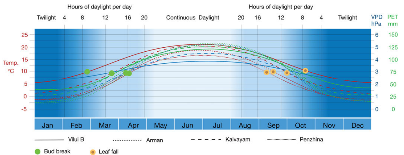
Fig. 5. Light, thermal and humidity regime for fossil assemblages at palaeolatitude ~70° N.
