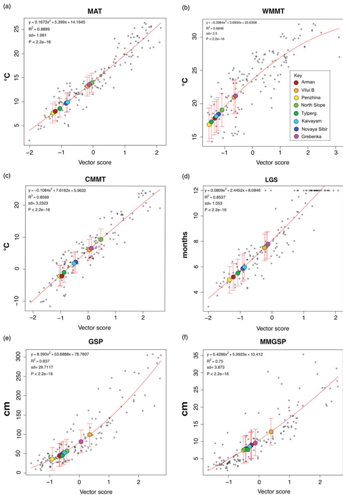
Fig. 6. CLAMP regression models for the WorldClim2_3brc modern vegetation calibration sites (open black circles) and predicted climate variables for eight early Late Cretaceous fossil sites (coloured circles as in the key shown in B). Bars indicate \pm 1 s.d. MAT – mean annual temperature; WMMT – warm month mean temperature; CMMT – cold month mean temperature; LGS – length of the growing season (temp. >10 °C); GSP – growing season precipitation; MMGSP – mean monthly growing season precipitation.
