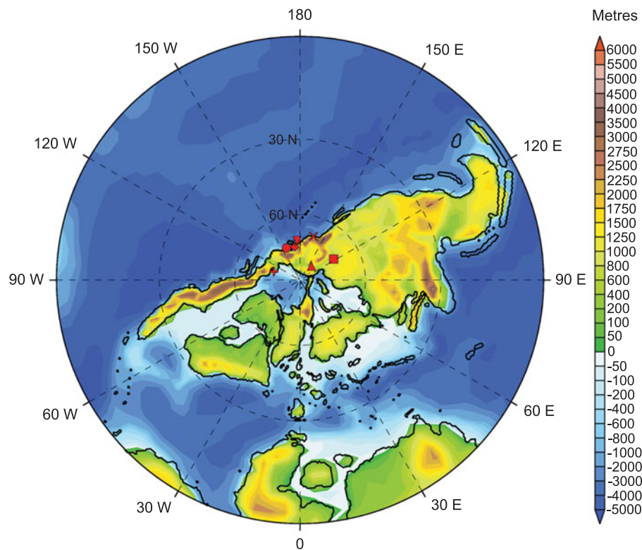
Fig. 2. North Polar projection of Turonian palaeogeography based on Getech Plc. reconstructions. Positions of fossil localities indicated by the following symbols: square – Vilui River; diagonal cross – Arman River; triangle – Novaya Sibir (New Siberia Island); inverted triangle – Grebenka River; diamond – Penzhina; star (partly hidden by the diamond) – Kaivayam; circle – Tylpergyrynai; horizontal cross – North Slope.
