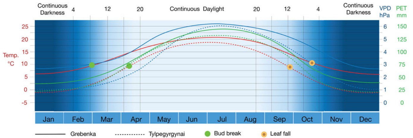
Fig. 4. Light, thermal and humidity regime for fossil assemblages at palaeolatitude ~75° N.
