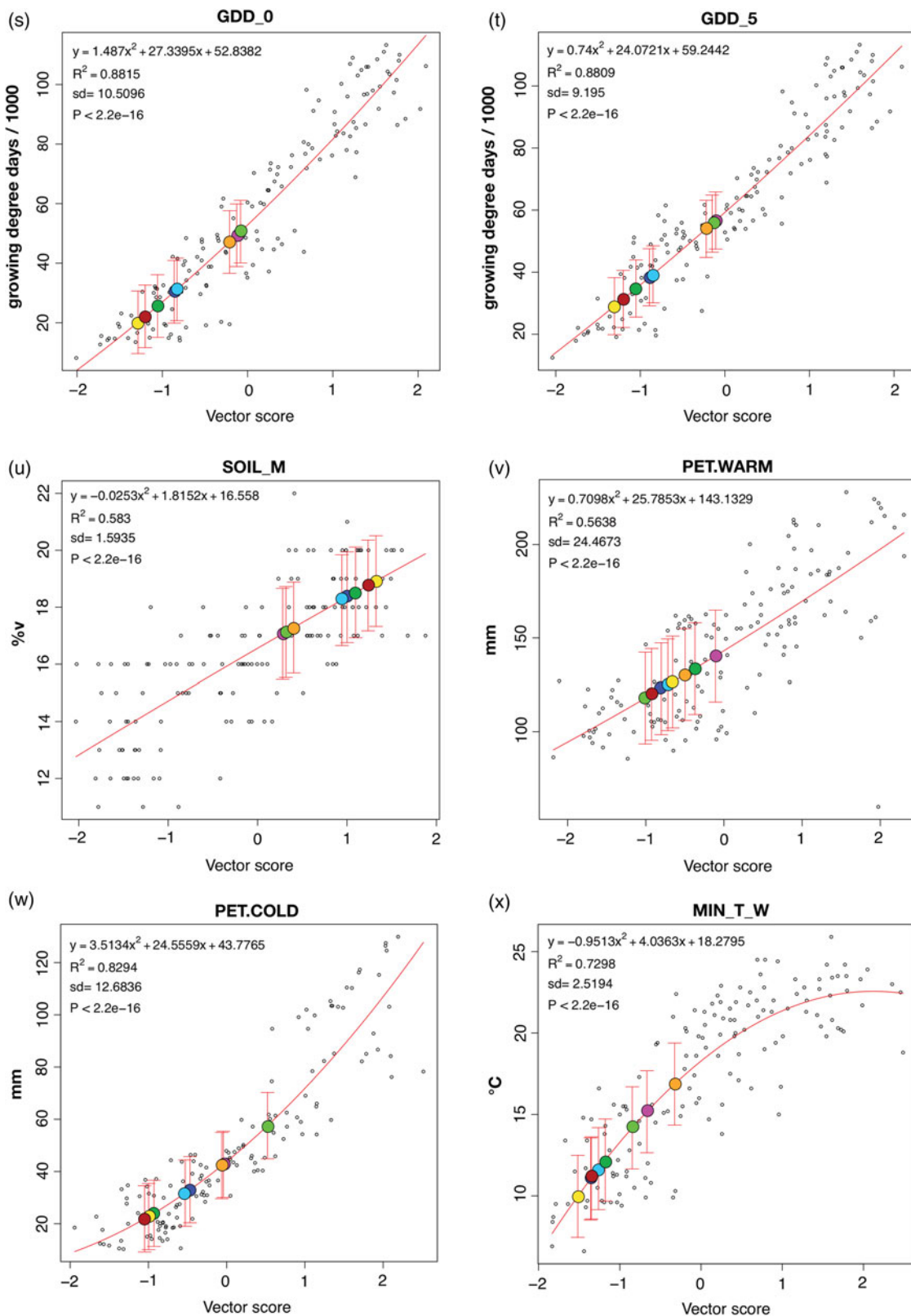
Fig. 9. CLAMP regression models for the WorldClim2_3brc modern vegetation calibration sites (open black circles) and predicted climate variables for eight early Late Cretaceous fossil sites (coloured circles as in the key shown in Fig. 6b). GDD_0 – growing degree days when temperatures are above freezing; GDD_5 – growing degree days when temperatures are above +5 °C; SOIL_M – derived soil moisture capacity; PET.WARM – potential evapotranspiration during the warmest month; PET.COLD – potential evapotranspiration during the coldest month; MIN_T_W – minimum temperature of the warmest month.
