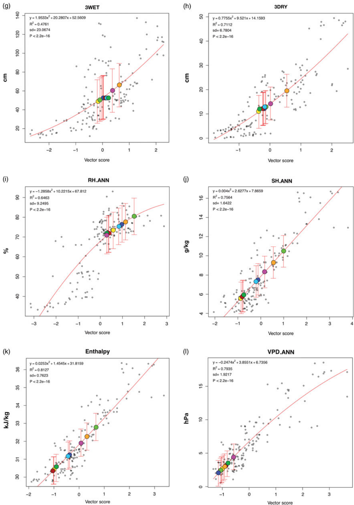
Fig. 7. CLAMP regression models for the WorldClim2_3brc modern vegetation calibration sites (open black circles) and predicted climate variables for eight early Late Cretaceous fossil sites (coloured circles as in the key shown in Fig. 6b). 3WET – precipitation in the three consecutive wettest months; 3DRY – precipitation in the three consecutive driest months; RH.ANN – mean annual relative humidity; SH.ANN – mean annual specific humidity; ENTH – mean annual moist enthalpy; VPD.ANN – mean annual vapour pressure deficit.
