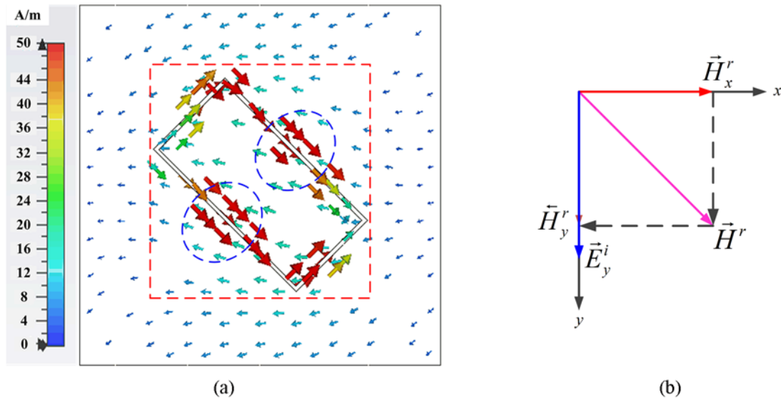
Figure 2. Induced current distribution of rectangular ring PCPS at 5.8 GHz and its decomposition diagram.
