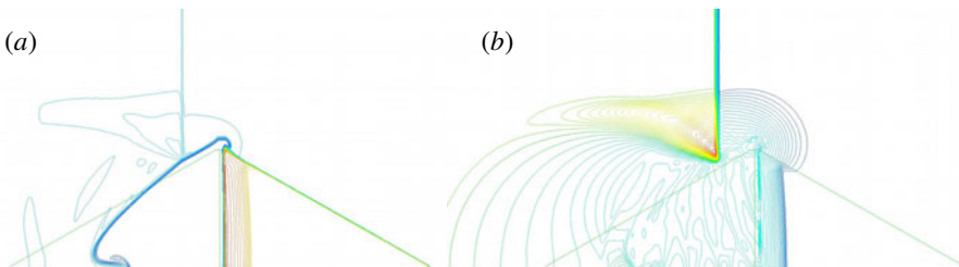
FIGURE 15. Wave pattern at t = 122 \mu\text{s} : (a) lines of constant density, and (b) lines of constant pressure.
