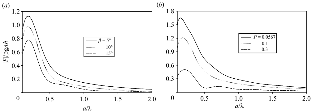
FIGURE 12. Hydrodynamic loading on (a) a submerged inclined porous plate as a function of a/\lambda and inclined angle for P = 0.1 , a/h = 2.0 , \theta = 0^\circ , and (b) a submerged horizontal porous plate as a function of a/\lambda and porosity for d/h = 0.1 , a/h = 2.0 , \theta = 0^\circ .
