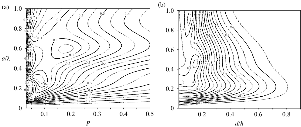
FIGURE 7. (a) Contour plots of reflection coefficients as a function of porosity ( P ) and a/\lambda for d/h = 0.1 , a/h = 1.0 , \theta = 0^\circ . (b) Contour plots of reflection coefficients as a function of submergence depth ( d/h ) and a/\lambda for P = 0.1 , a/h = 1.0 , \theta = 0^\circ
