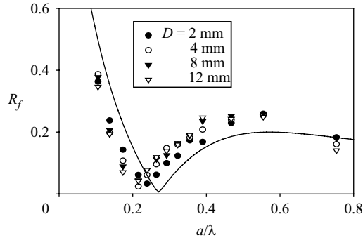
FIGURE 6. Comparison of analytic and experimental results for a horizontal punched plate with a vertical wall as a function of a/\lambda and hole size ( P = 0.1008 , a/h = 1.0 , d/h = 0.025 , \theta = 0^\circ ). — calculation.
